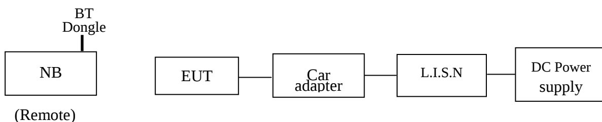
Fig. 2-2 Configuration of Tested System (DC Power Line Conducted Test)
