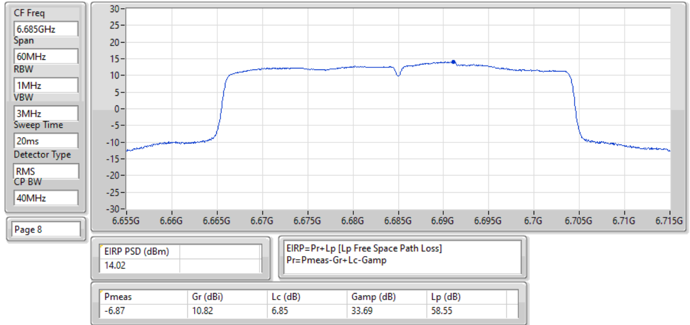
EIRP PSD;Band:6.7G;ax40;BWch:40MHz;Nss:1,(M0);Nant:1(2);Ch:6685MHz;TX
