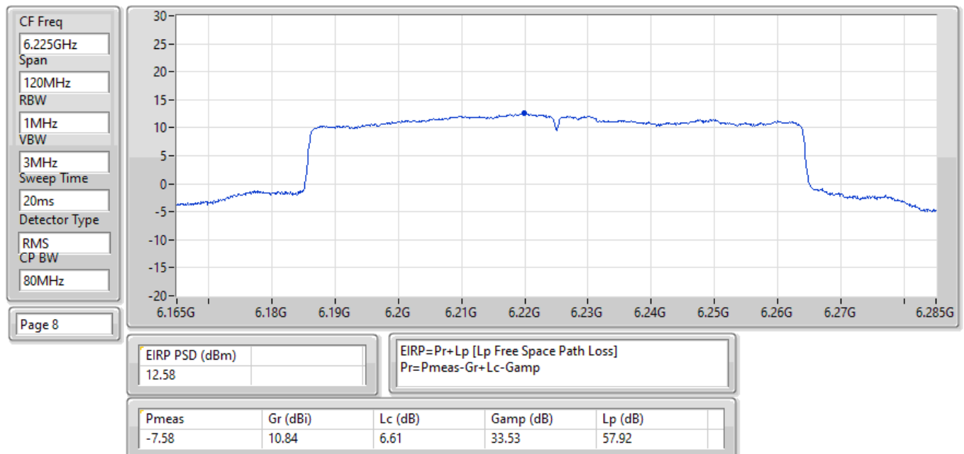
EIRP PSD;Band:6.2G;ax80;BWch:80MHz;Nss:1,(M0);Nant:1(2);Ch:6225MHz;TX
