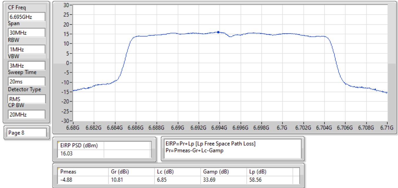
EIRP PSD;Band:6.7G;ax20;BWch:20MHz;Nss:1,(M0);Nant:1(2);Ch:6695MHz;TX
