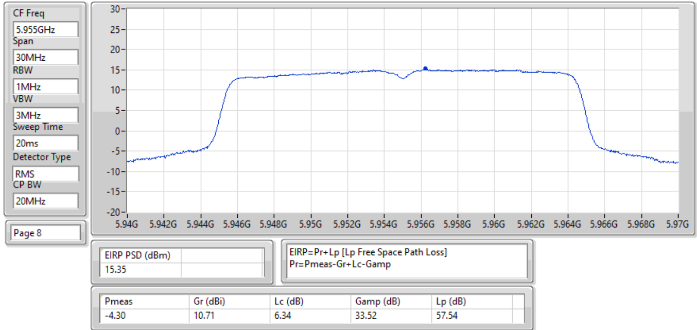
EIRP PSD;Band:6.2G;ax20;BWch:20MHz;Nss:1,(M0);Nant:1(2);Ch:5955MHz;TX
