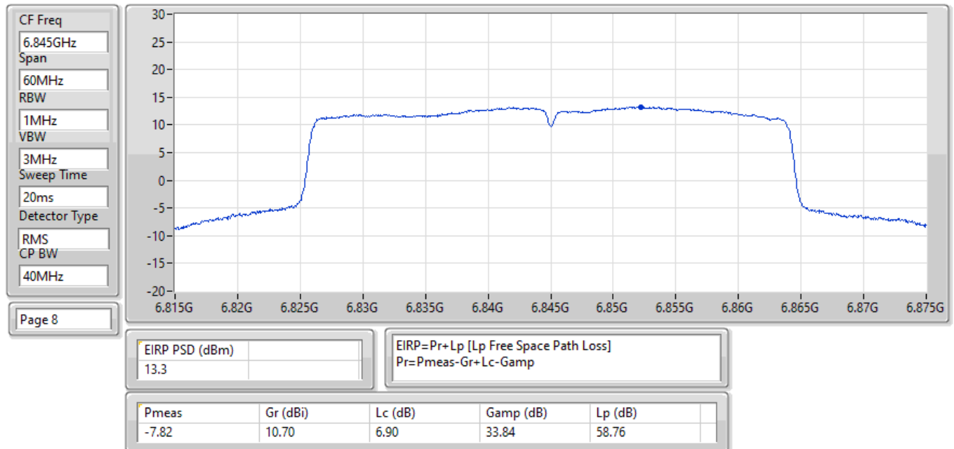
EIRP PSD;Band:6.7G;ax40;BWch:40MHz;Nss:1,(M0);Nant:1(2);Ch:6845MHz;TX
