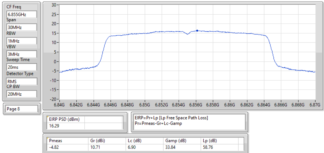
EIRP PSD;Band:6.7G;ax20;BWch:20MHz;Nss:1,(M0);Nant:1(2);Ch:6855MHz;TX
