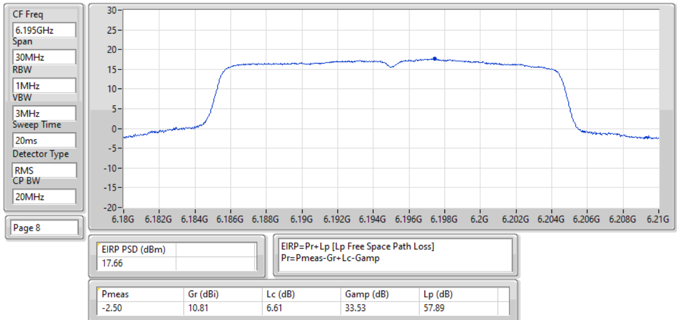
EIRP PSD;Band:6.2G;ax20;BWch:20MHz;Nss:1,(M0);Nant:1(2);Ch:6195MHz;TX
