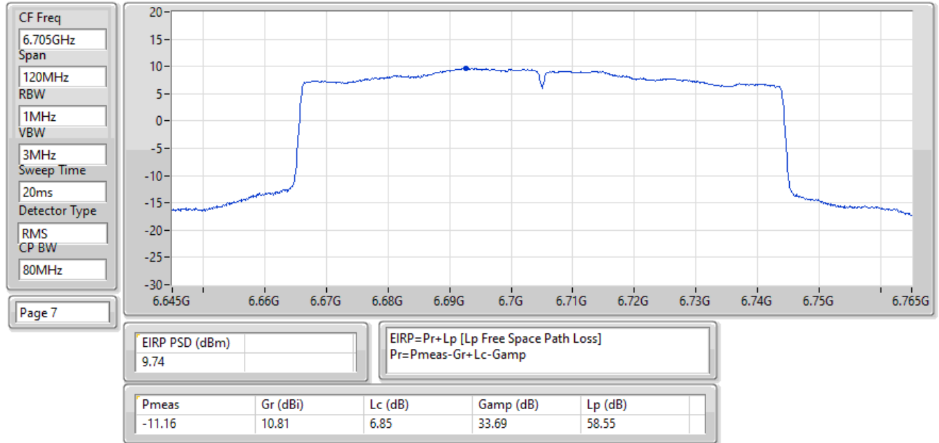
EIRP PSD;Band:6.7G;ax80;BWch:80MHz;Nss:1,(M0);Nant:1(2);Ch:6705MHz;TX
