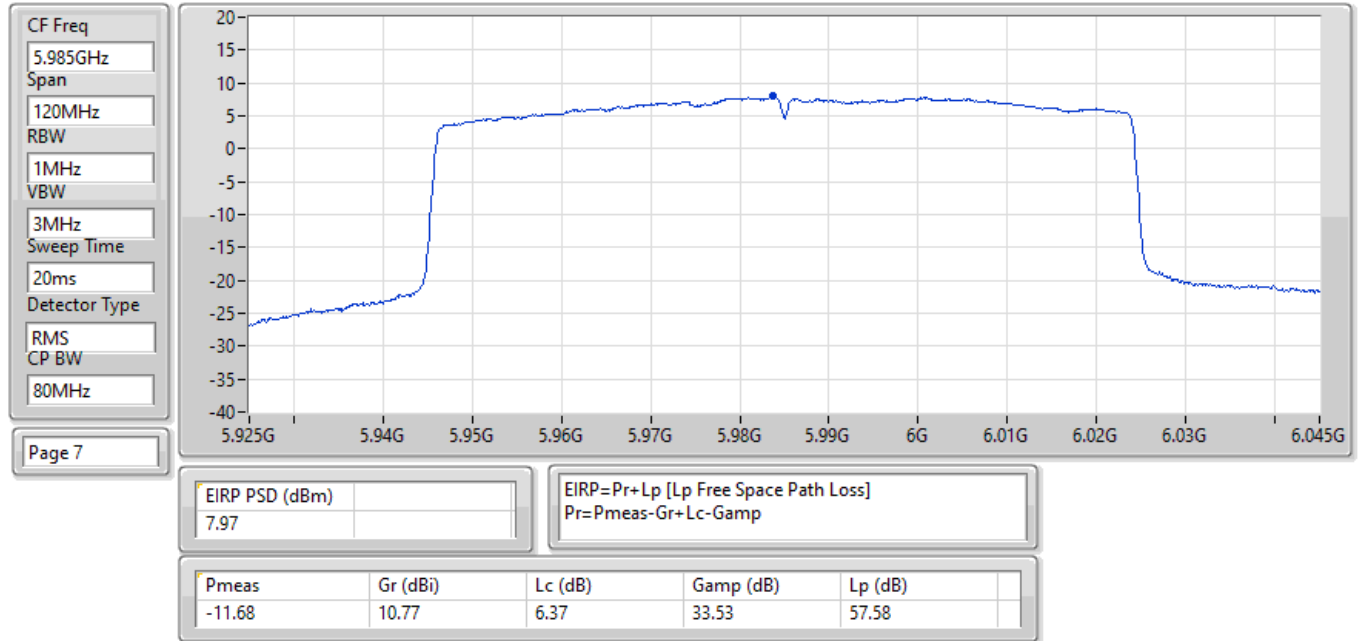
EIRP PSD;Band:6.2G;ax80;BWch:80MHz;Nss:1,(M0);Nant:1(2);Ch:5985MHz;TX
