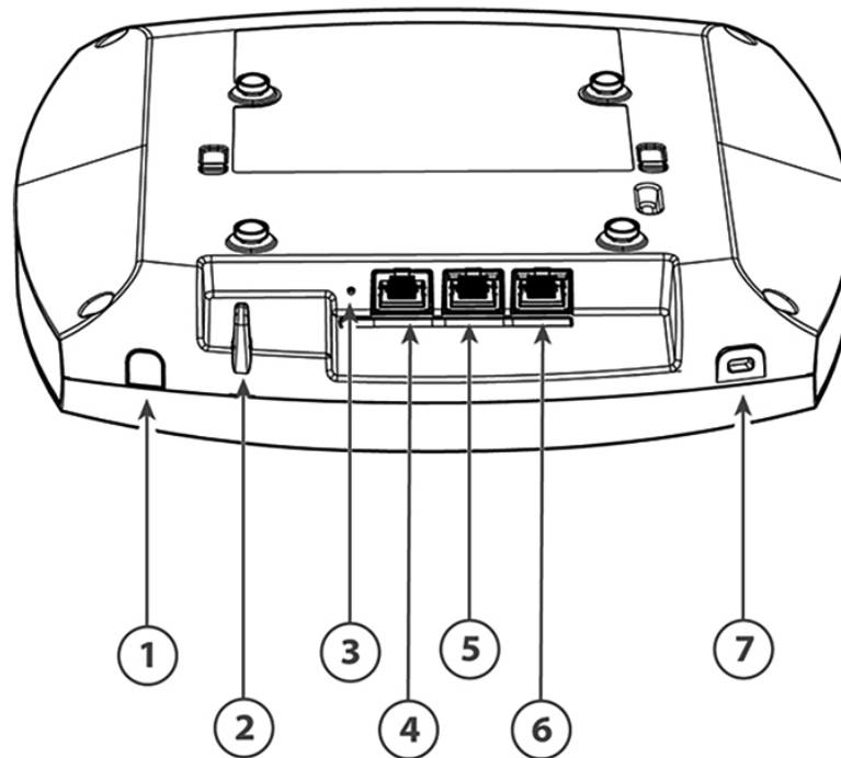
Figure 2: CW9178I Top View with Connectors and Ports
