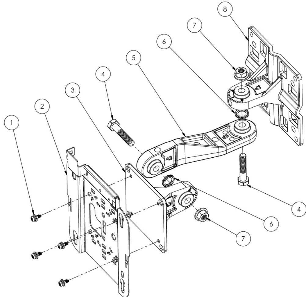
Figure 3: Exploded View of the Wall Mounting Articulating Bracket Hardware Assembly
