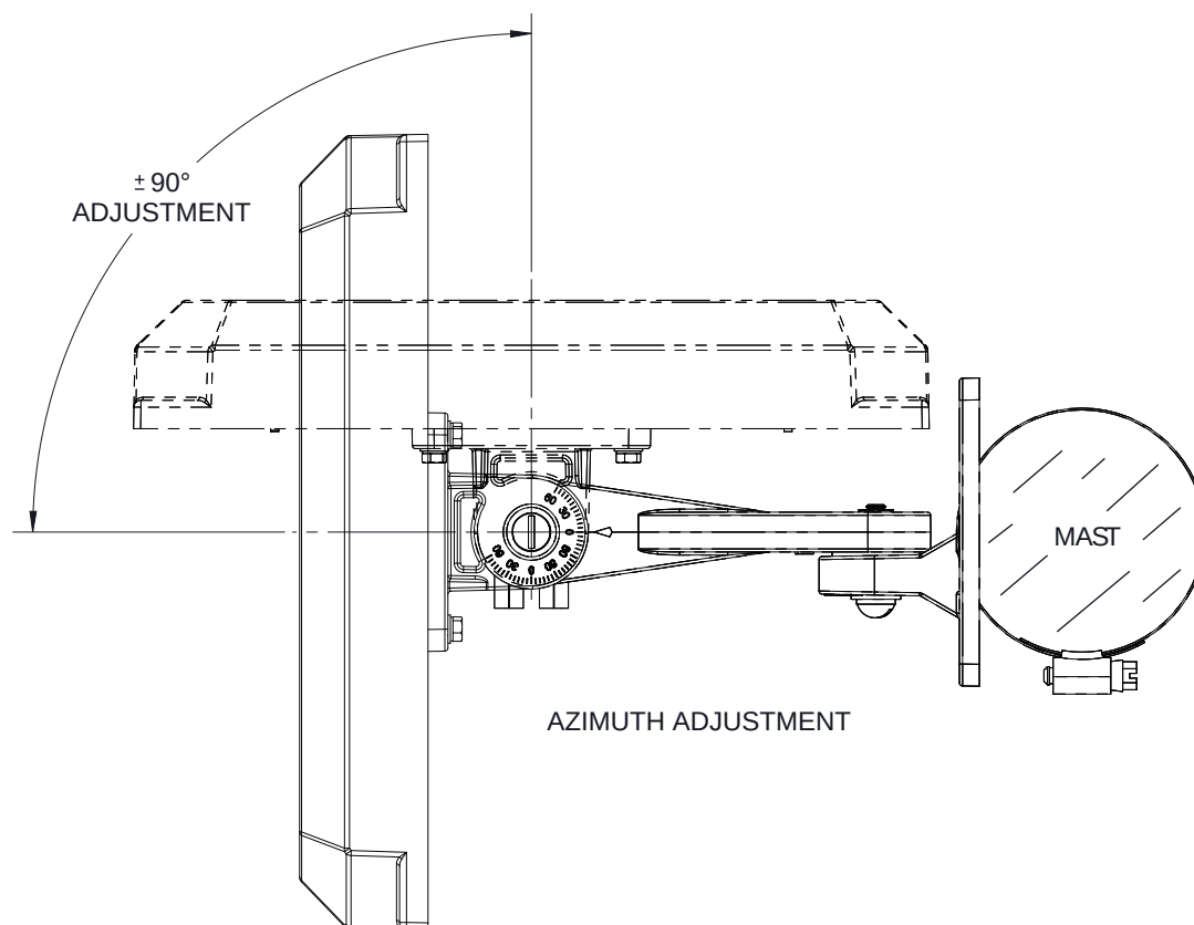
Figure 7 Azimuth Adjustment
