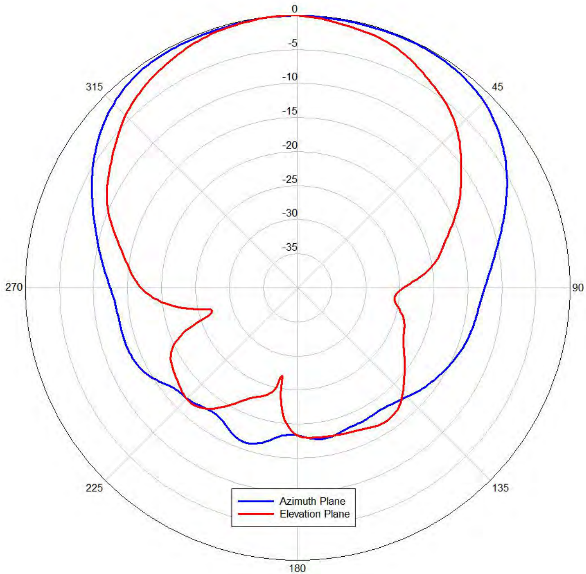
Figure 1 Azimuth and Elevation Radiation Patterns - 2.4 GHz Band
