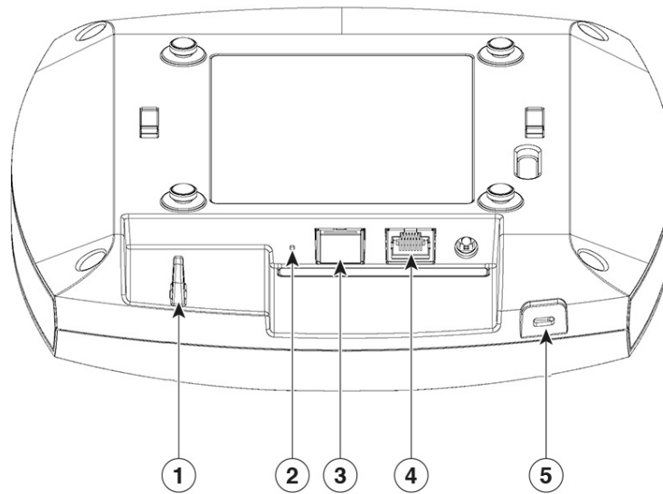
Figure 2: CW9174I Top View with Connectors and Ports
