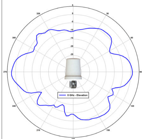
5 GHz - Elevation- Port E
