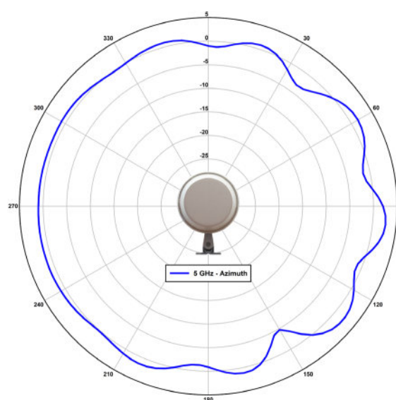
5 GHz - Azimuth - Port E
