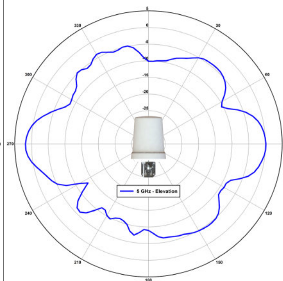
5 GHz - Elevation- AUX Port
