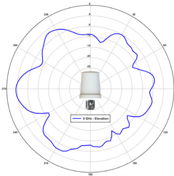
5 GHz - Elevation- Port H
