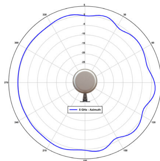
5 GHz - Azimuth - AUX Port
