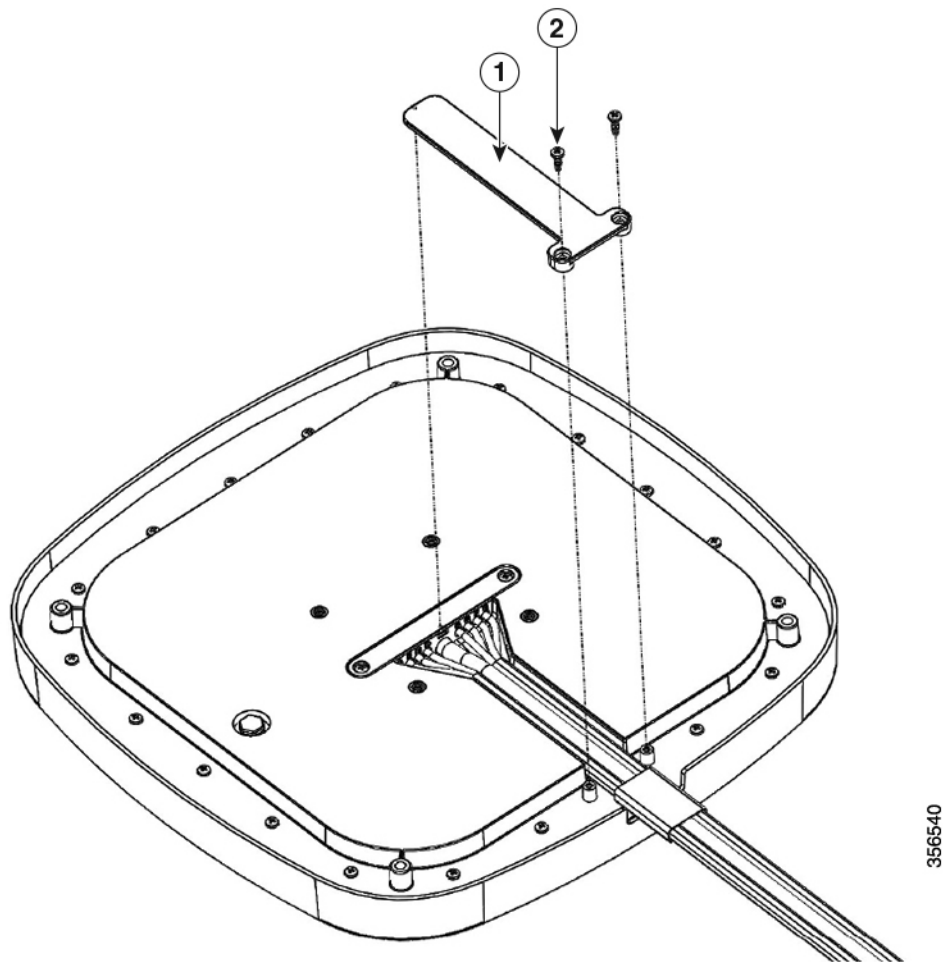
Figure 6 Cable Restraint on the Back of the Antenna
