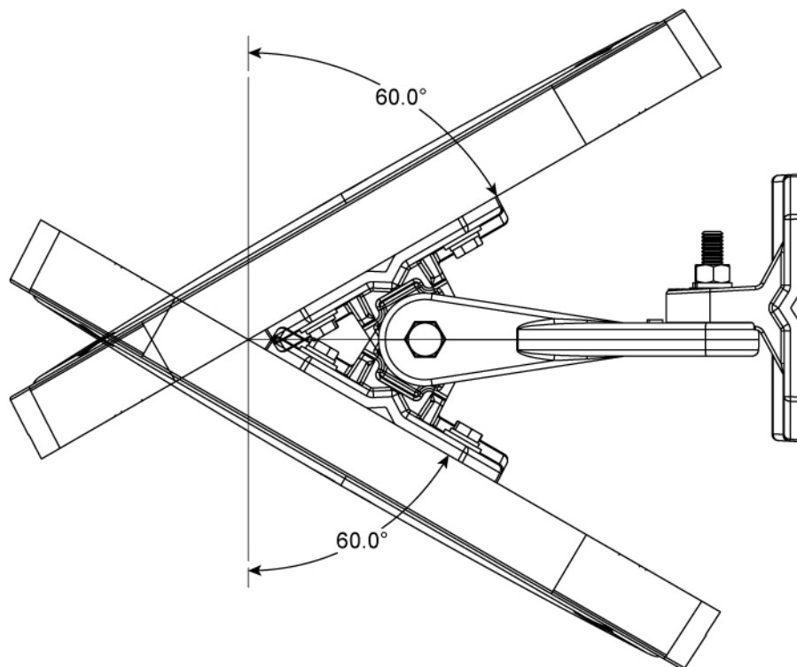
Figure 9 Elevation Adjustment
