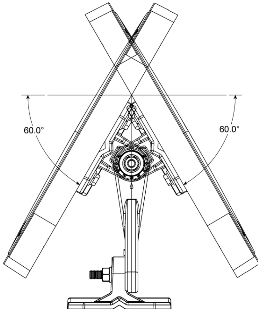
Figure 8 Azimuth Adjustment
