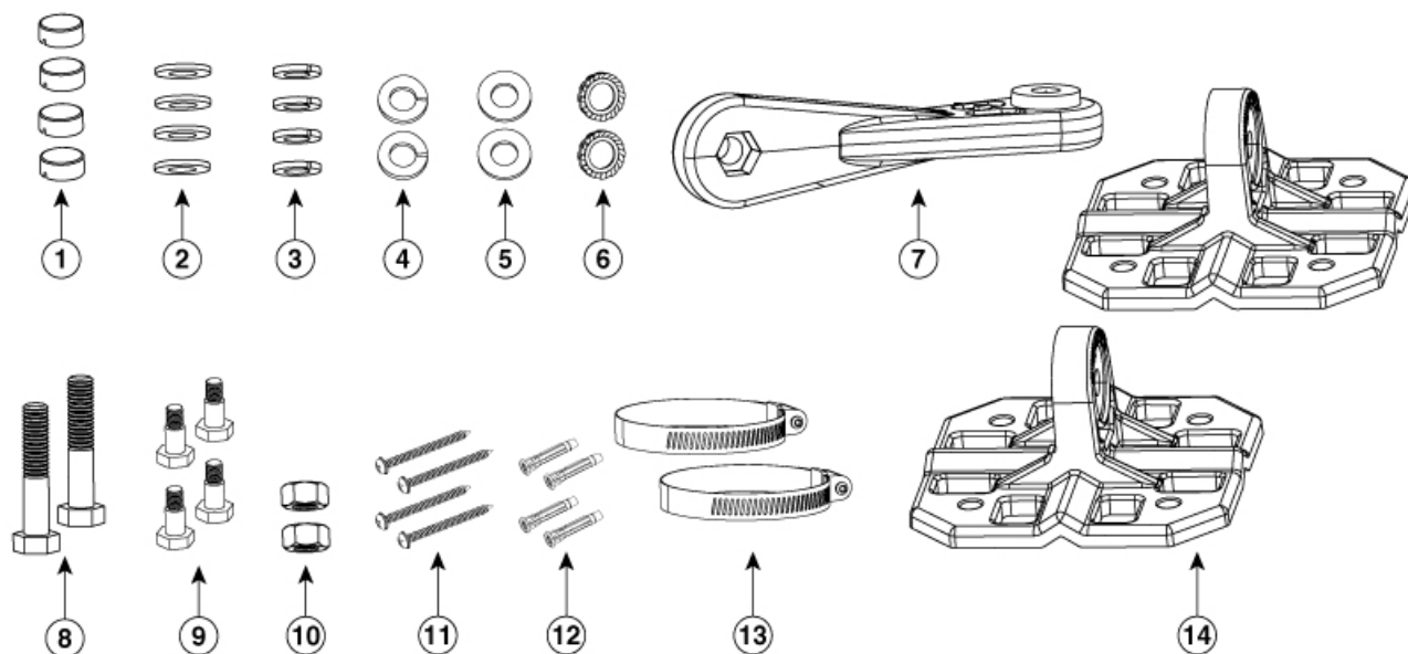
Figure 1 Contents of the Antenna Bracket Kit
