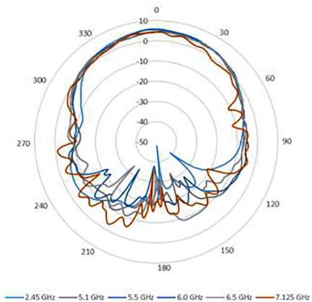
Azimuth - Port D
