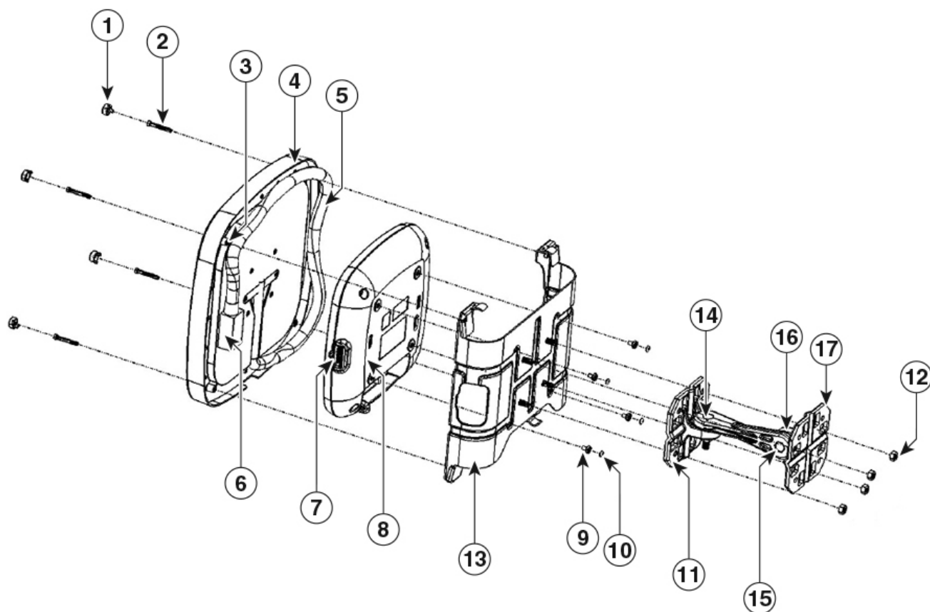
Figure 12 Exploded View of Bracket Hardware Assembly for Directly Mounting Access Point to Back of Antenna
