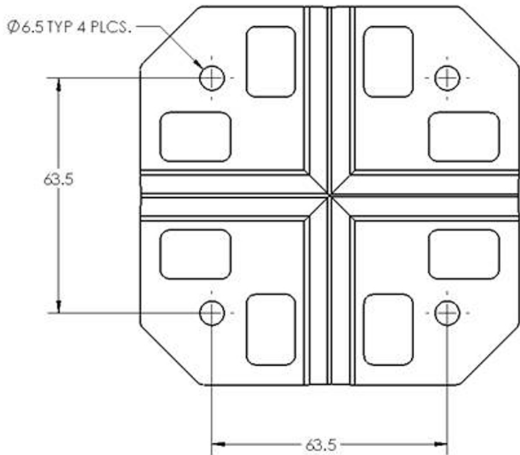
Figure 4 Locations of the Screw Holes on the Articulating Mount Flange
