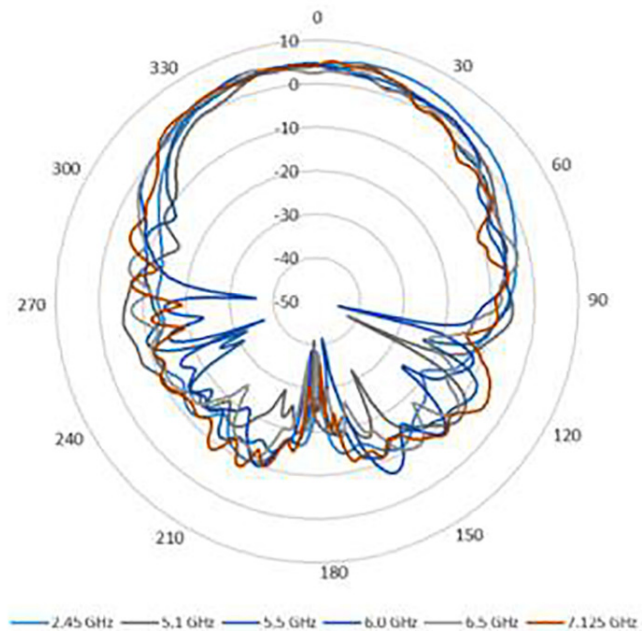
Azimuth - Port F
