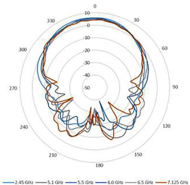
Elevation - Port D
