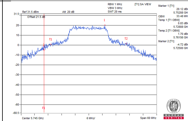
802.11a_Chain 3 / CH149
