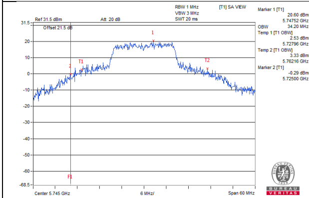
802.11a_Chain 2 / CH149
