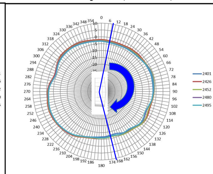
XY-plane (theta 90°)
