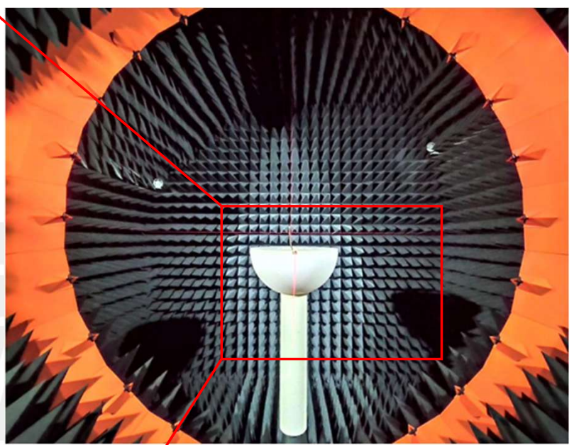
MVG SATIMO SG24L Anechoic Chamber
