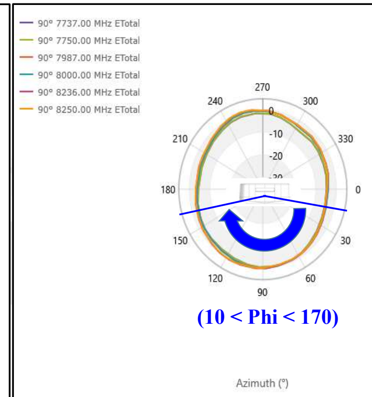
XY-plane (theta 90°)
