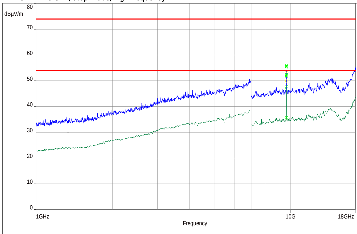
Plot 12: 1GHz – 18 GHz, stop mode, high frequency
