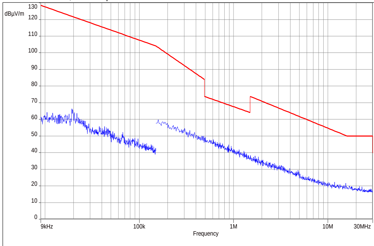
Plot 3: 9 kHz – 30 MHz, normal operation mode
