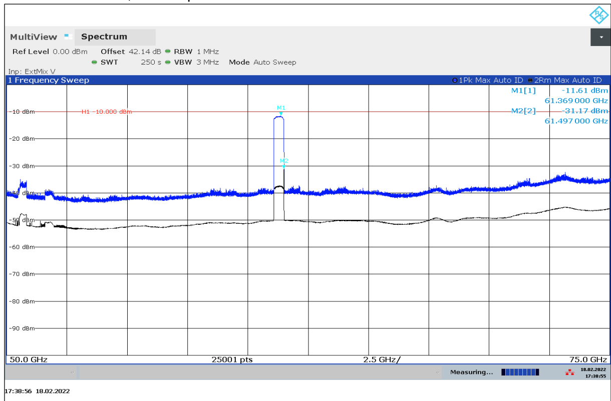
Plot 17: 50 GHz – 75 GHz, normal operation mode
