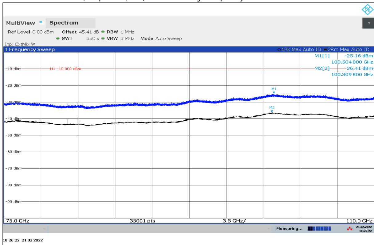
Plot 24: 75 GHz – 110 GHz, stop mode, low, middle and high frequency
