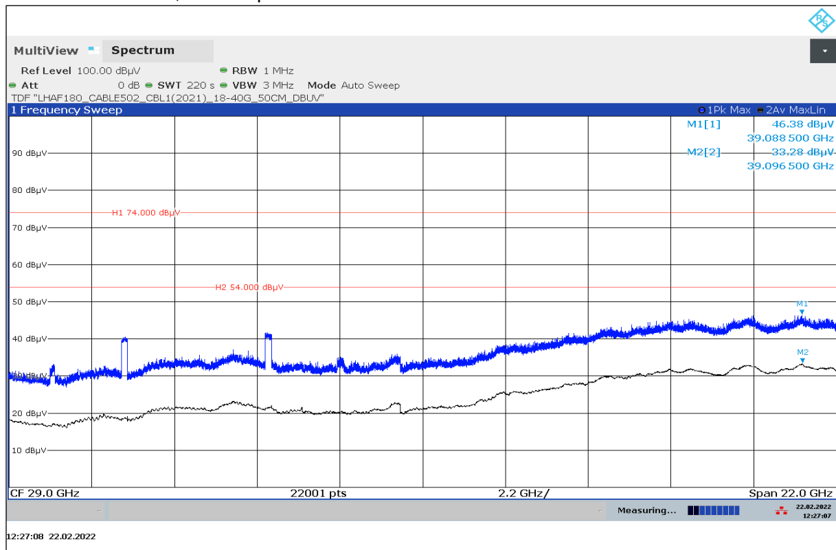
Plot 13: 18 GHz – 40 GHz, normal operation mode
