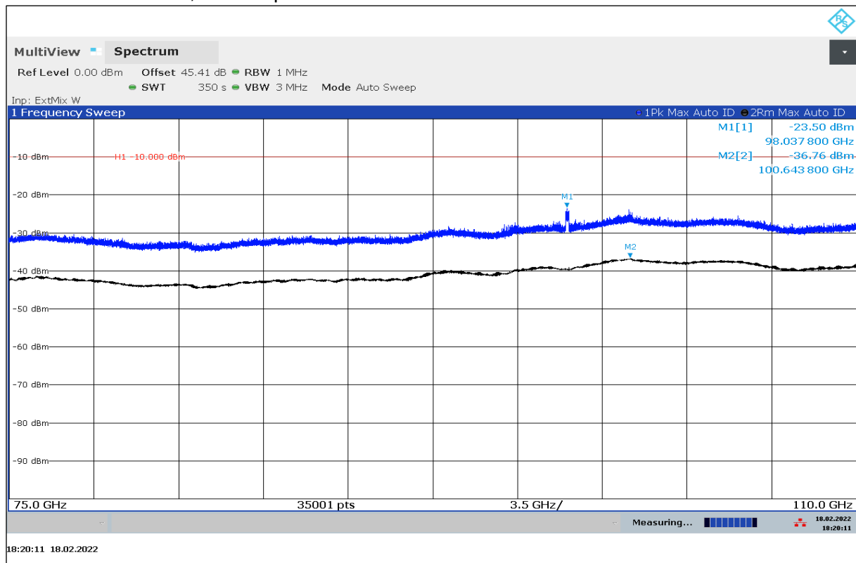
Plot 23: 75 GHz – 110 GHz, normal operation mode
