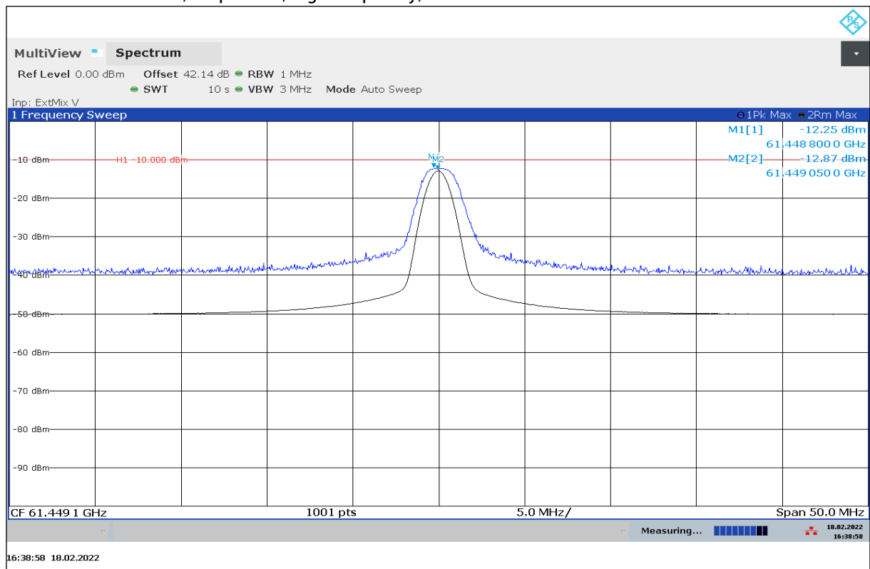
Plot 22: 50 GHz – 75 GHz, stop mode, high frequency, detail
