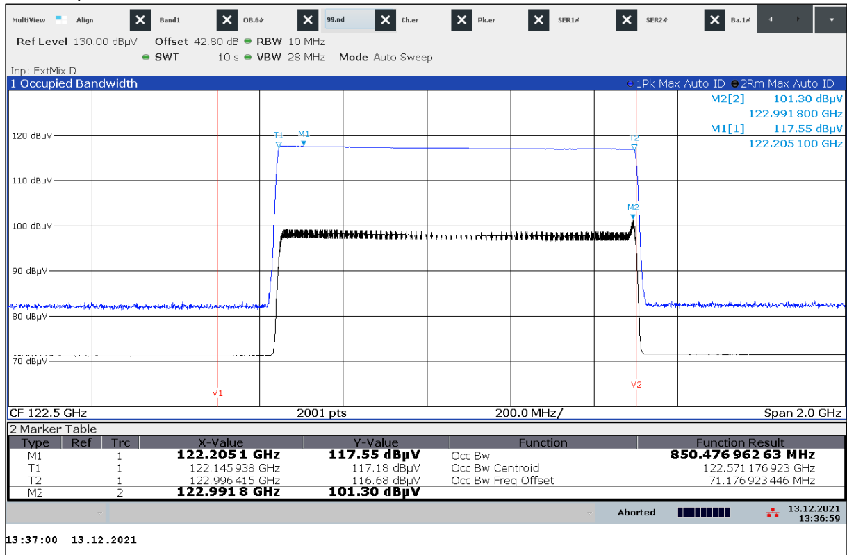
Plot 50: Occupied bandwidth, +40 °C / V nom
