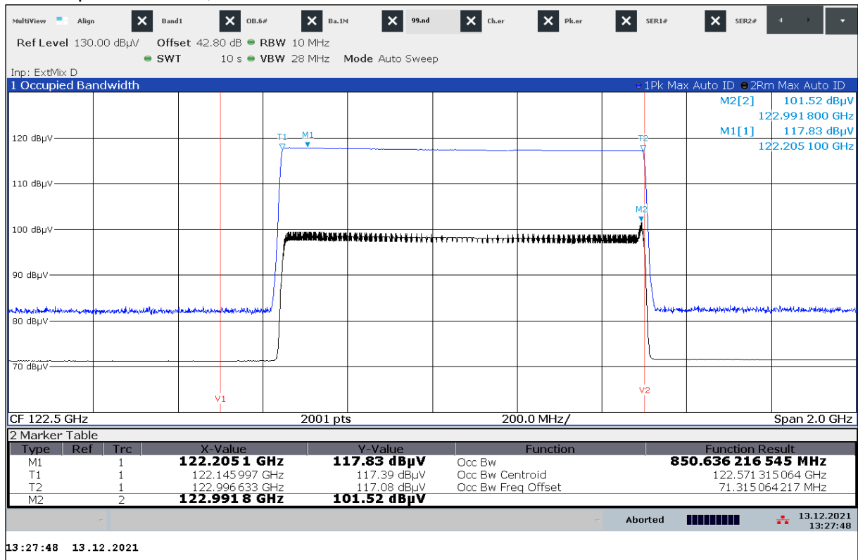
Plot 49: Occupied bandwidth, +30 °C / V_{\text{nom}}
