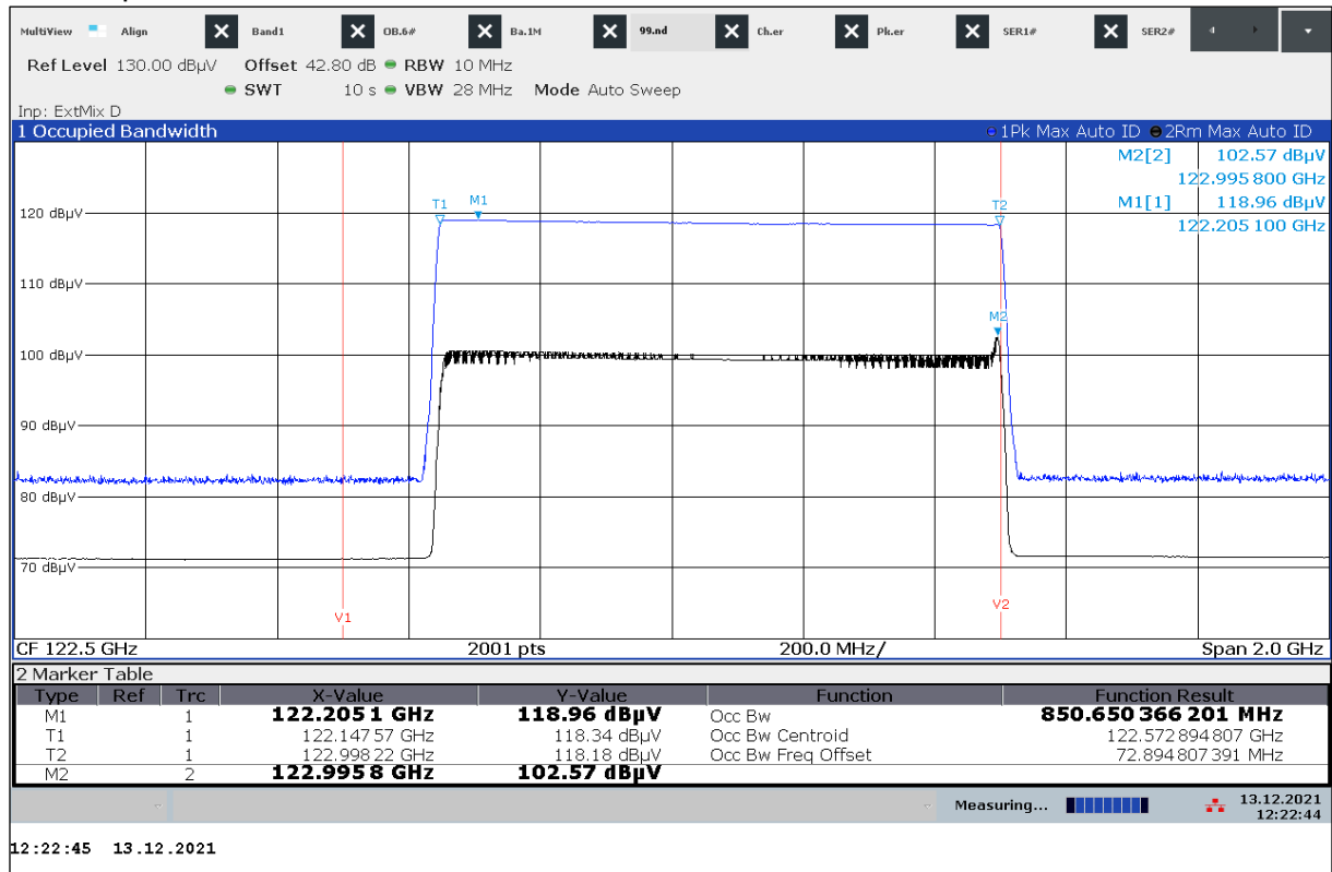
Plot 44: Occupied bandwidth, 0 °C / V_{nom}
