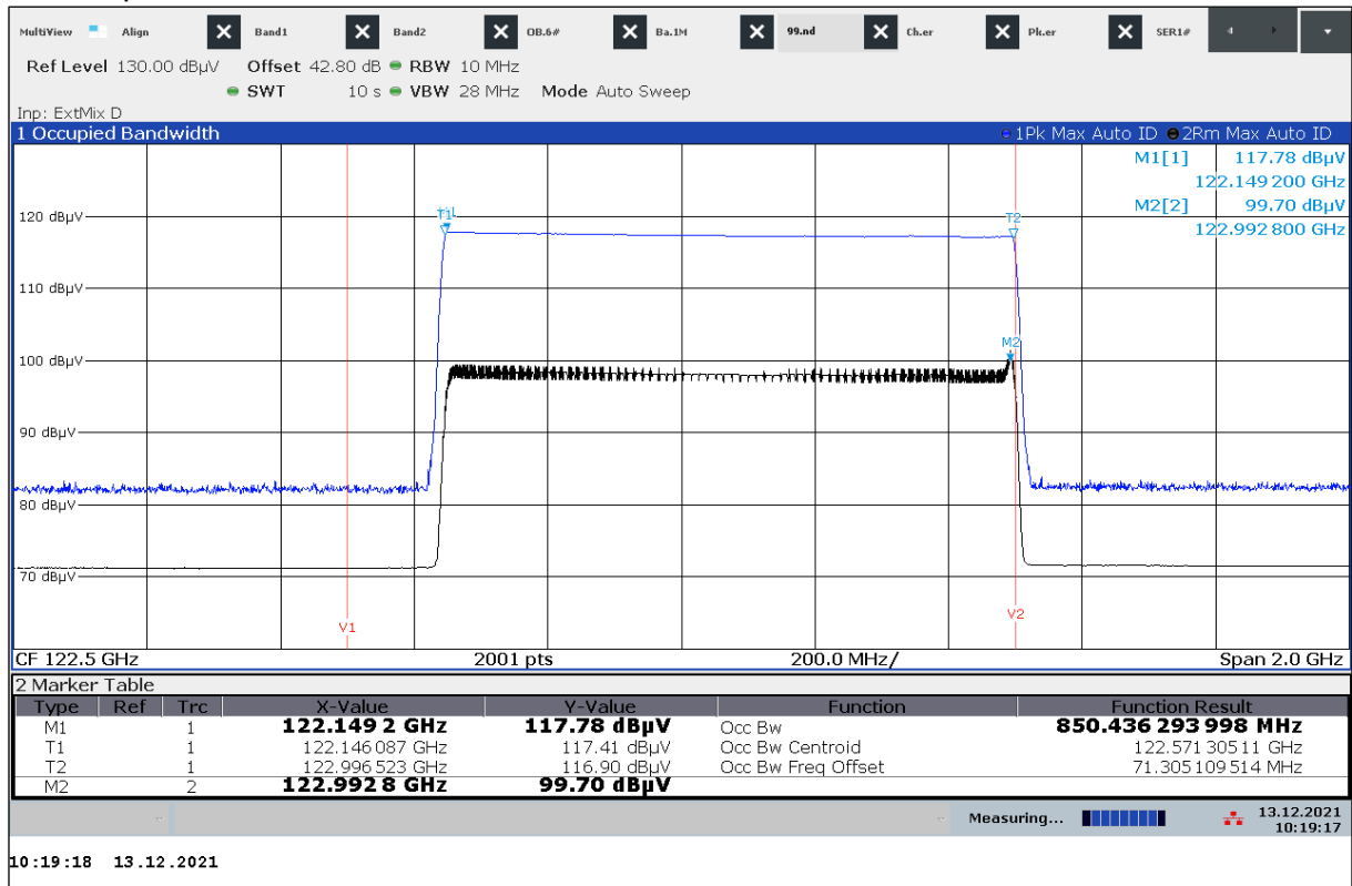
Plot 48: Occupied bandwidth, +20 °C / V_{\max}
