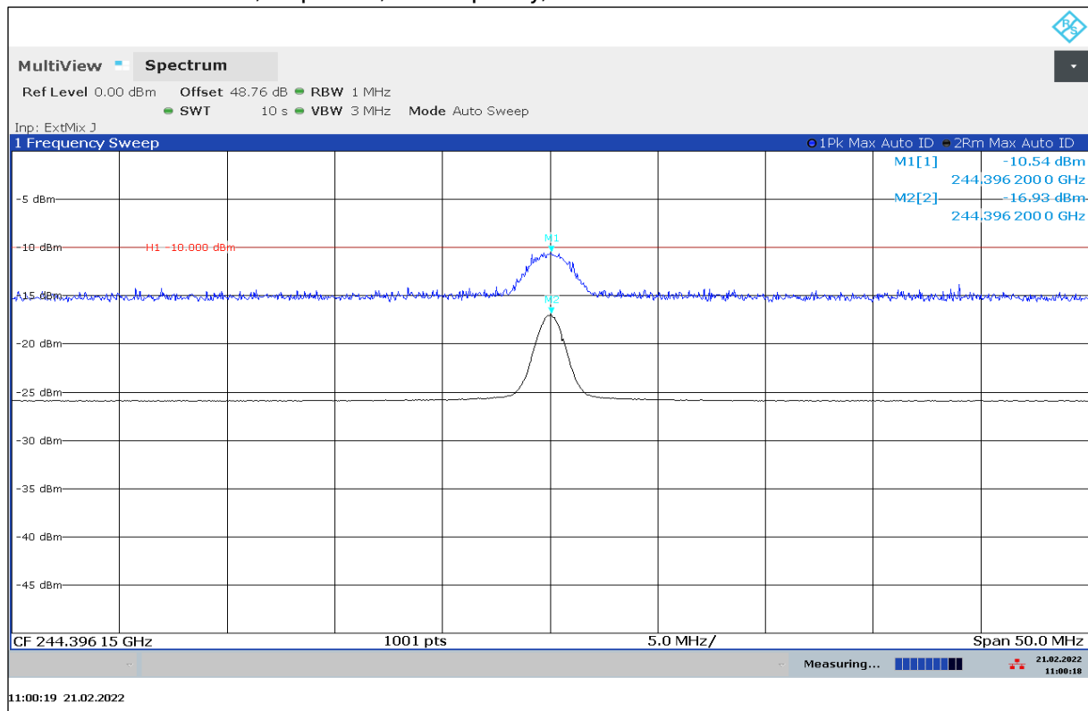
Plot 34: 220 GHz – 300 GHz, stop mode, low frequency, detail
