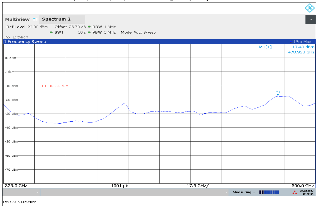
Plot 40: 325 GHz – 500 GHz, stop mode, low, middle and high frequency
