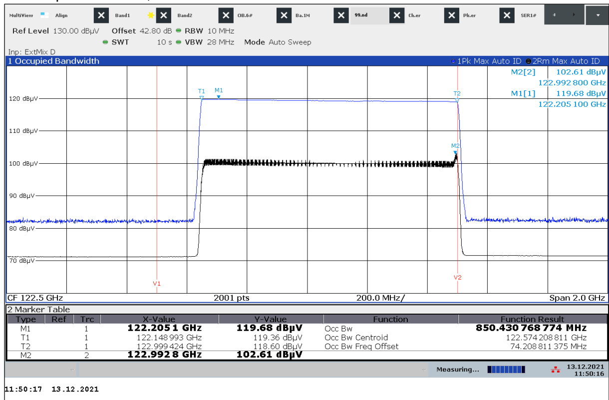
Plot 42: Occupied bandwidth, -20 °C / V nom
