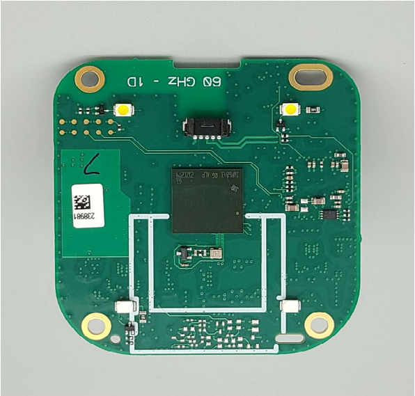
Dual Discrete - PCB 235290
