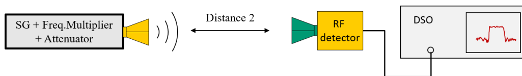
Fig. 2: Test setup 2. P_{\text{SG}} + \text{AG}_{\text{TX}} - \text{FSL}_2 + \text{AG}_{\text{meas}} = P_{\text{detector}}
