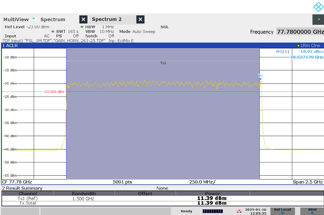
Plot 6: Channel power tested under nominal condition TnomVnom
