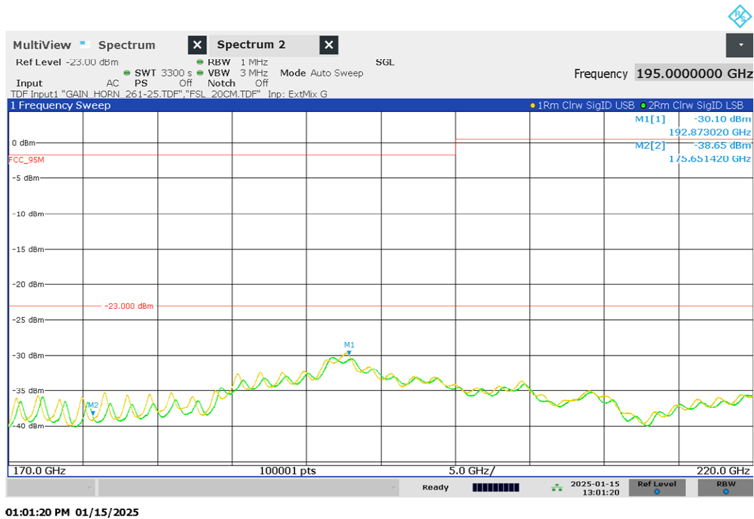
Plot 10: Radiated emissions 170 - 220 GHz
