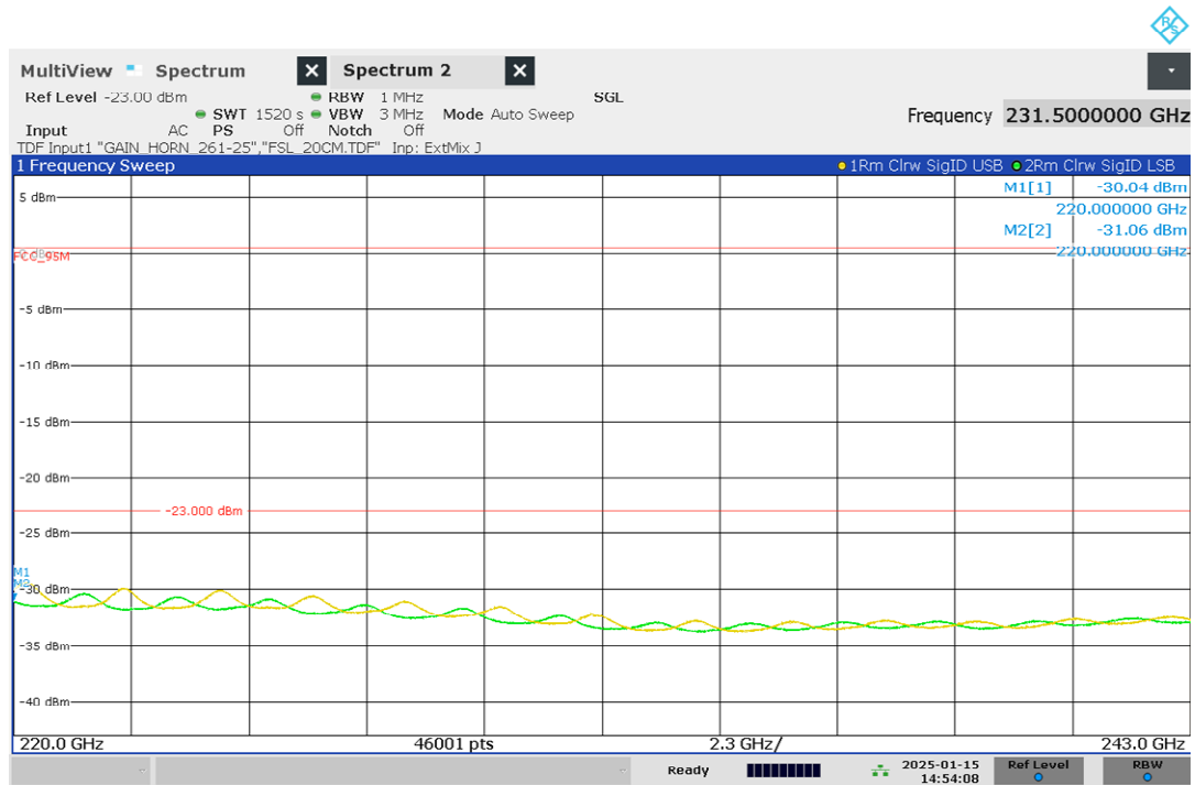
Plot 11: Radiated emissions 220 – 243 GHz
