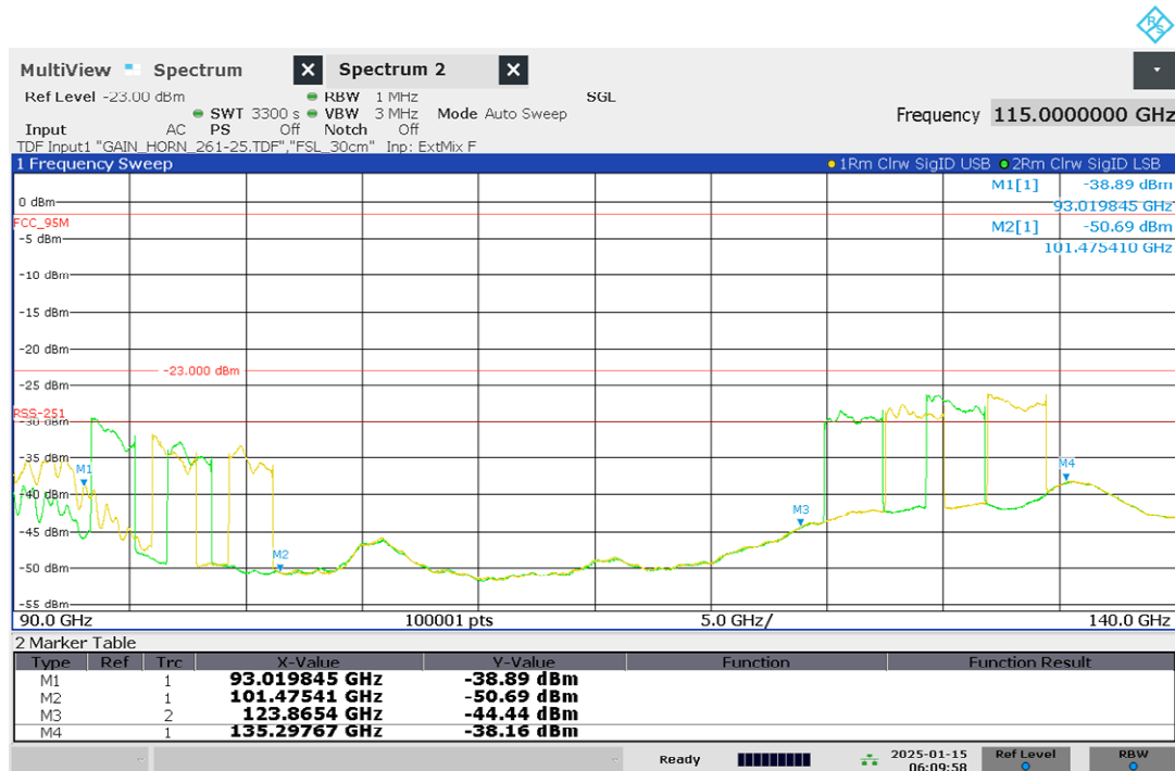
Plot 8: Radiated emissions 90 – 140 GHz
