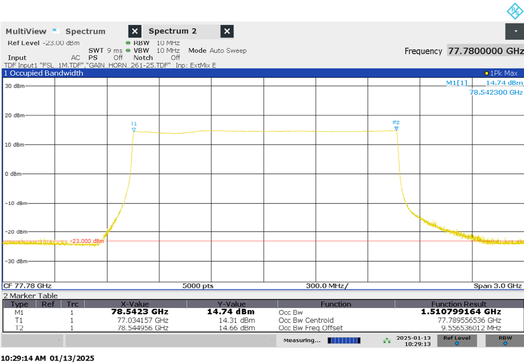
Plot 1: bandwidth per ISED requirement (RBW = 10 MHz)
