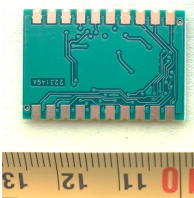
Figure 3: Back view
