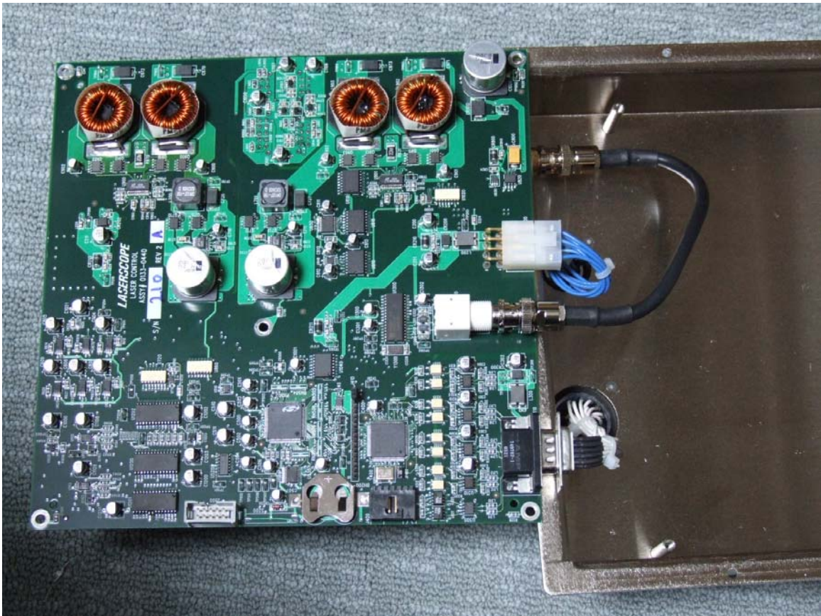
Board & Enclosure Component Side
