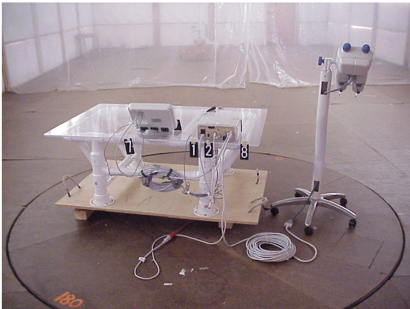
RADIATED EMISSIONS TEST SETUP / REAR VIEW
