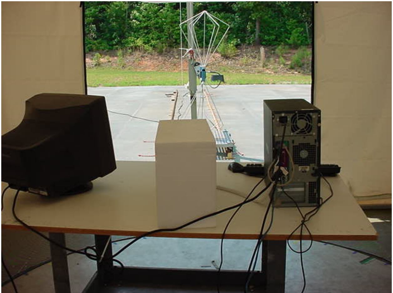
Figure 5: Radiated Emissions
