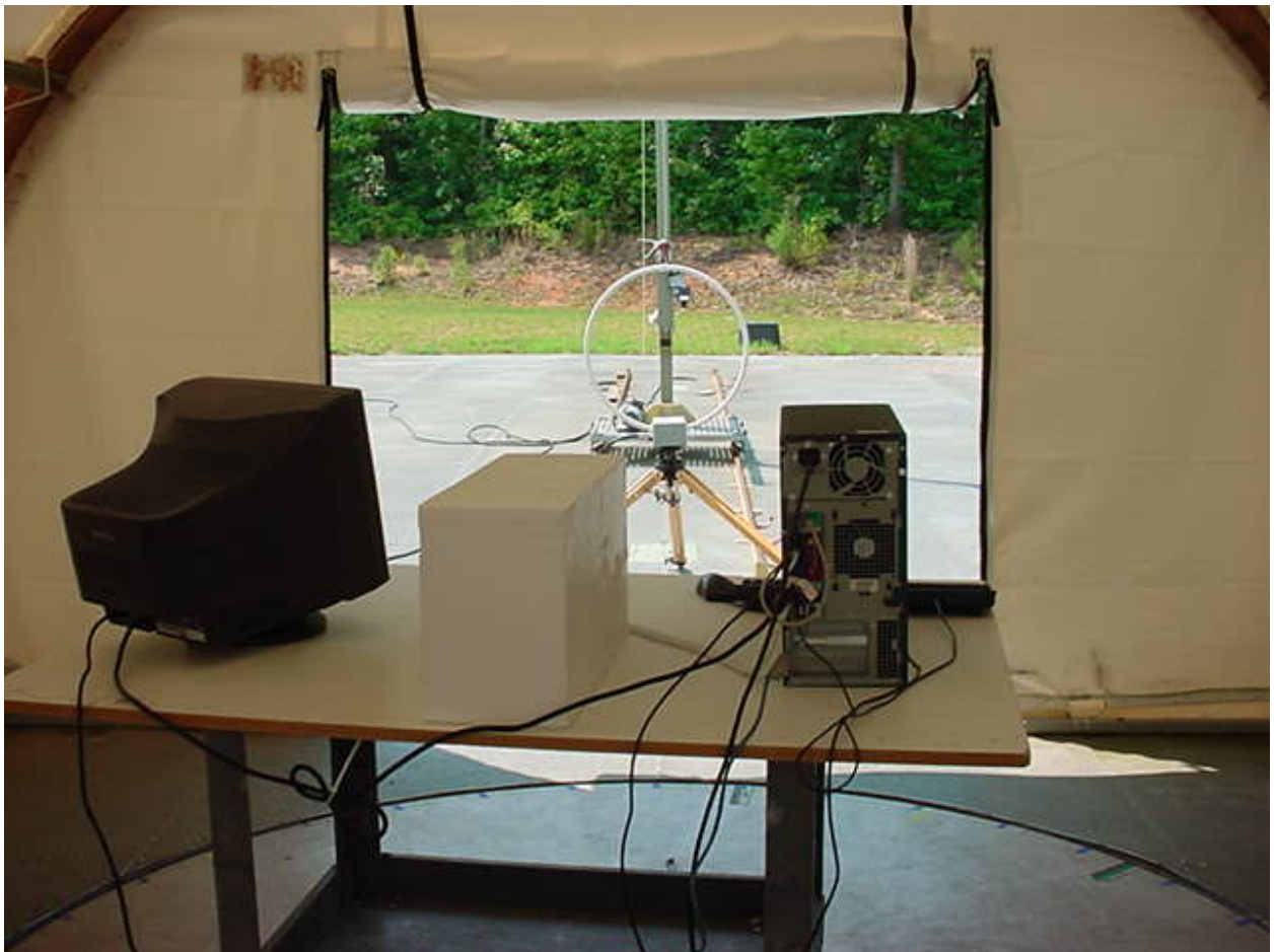
Figure 4: Radiated Emissions
