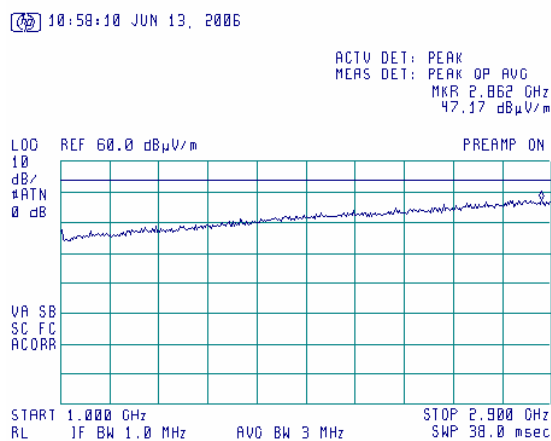
Plot 7.4.4 Radiated emission measurements in 1000 -2900 MHz, horizontal antenna polarization
