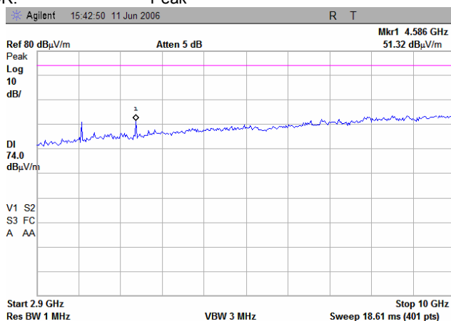
Plot 7.1.10 Radiated emission measurements from 2.9 to 10.0 GHz
