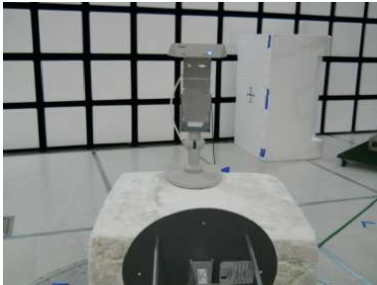
RADIATED EMISSIONS
