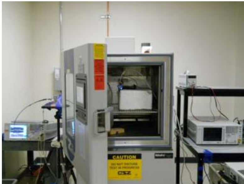
TEMPERATURE CHAMBER
