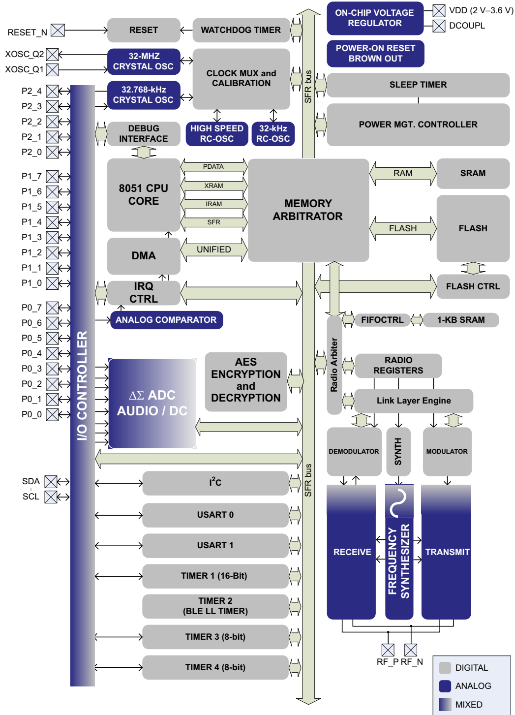
Figure 1. Block Diagram
