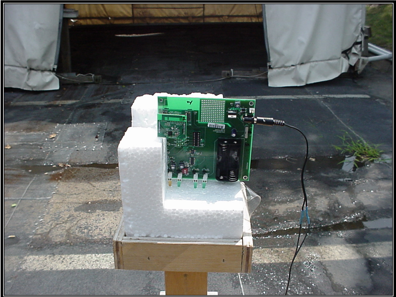
Photograph 4: Radiated Spurious/Harmonics Testing – Front View
