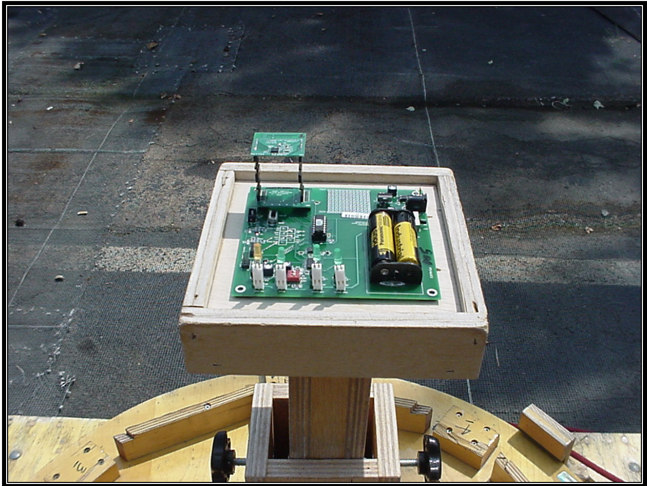
Photograph 2: Radiated Digital Testing – Front View
