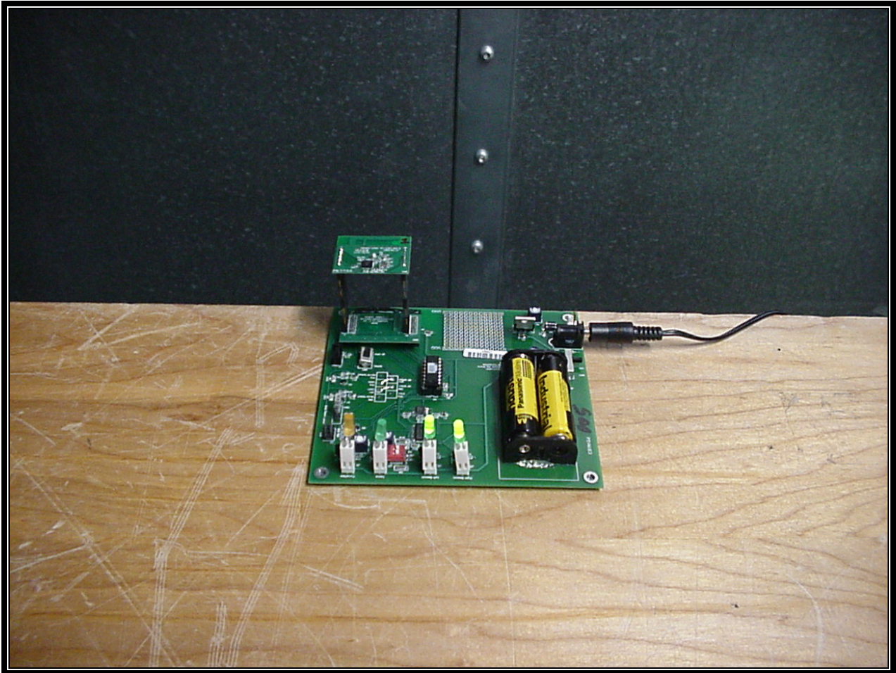
Photograph 6: AC Conducted Emissions Testing – Front View
