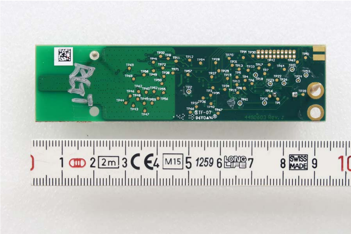
PCB Rear
