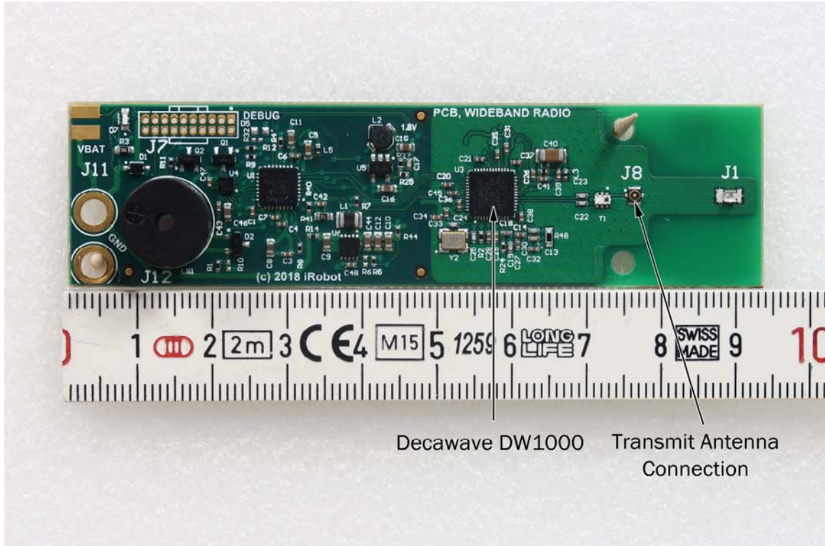
PCB Front
