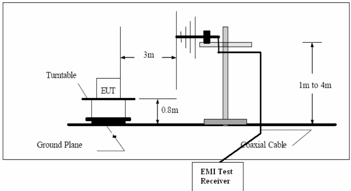
Figure 2 Radaited test setup
