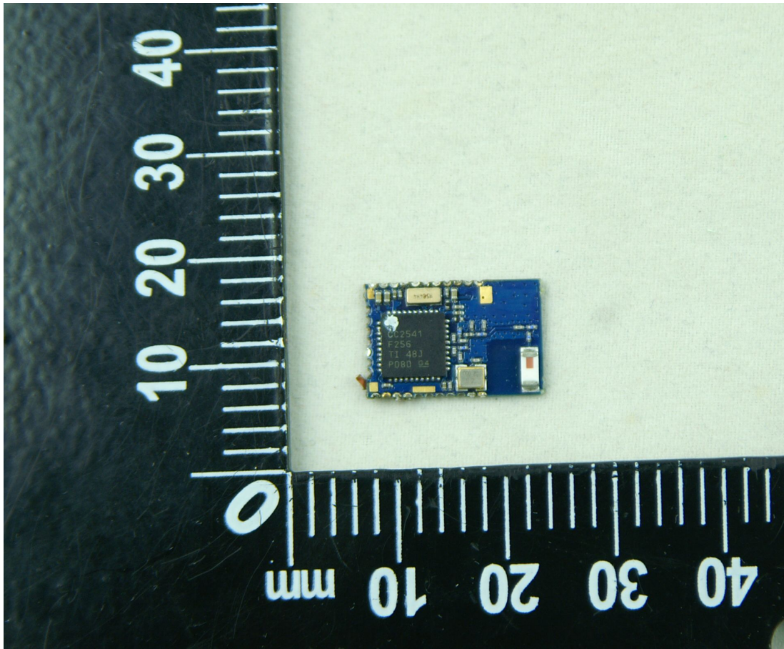
THE PHOTO OF RF CHIP 1
