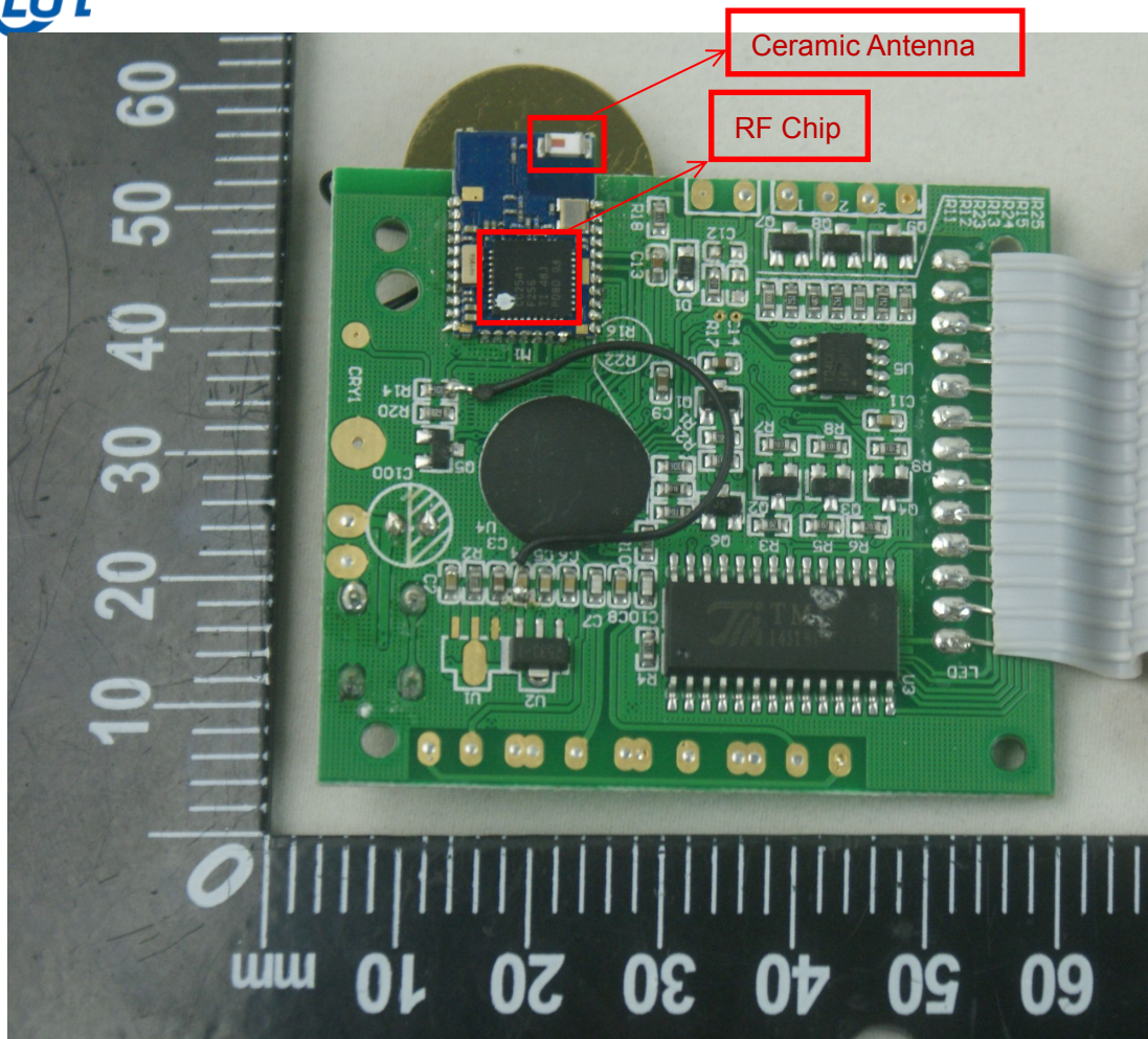
MAIN BOARD BACK VIEW 2
