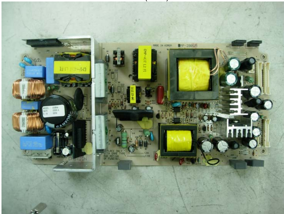
SMPS (Rear)
