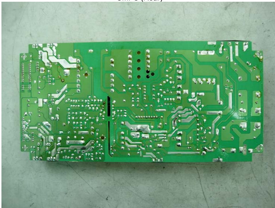
SMPS (Rear)
