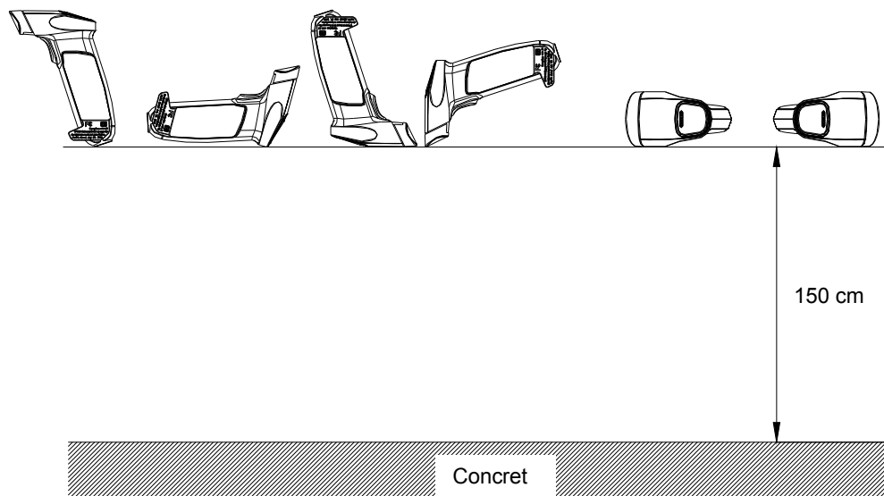
Figure 10: Drop Test
