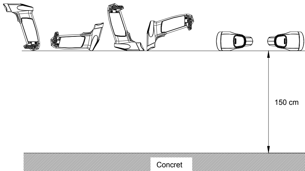
Figure 10: Drop Test
