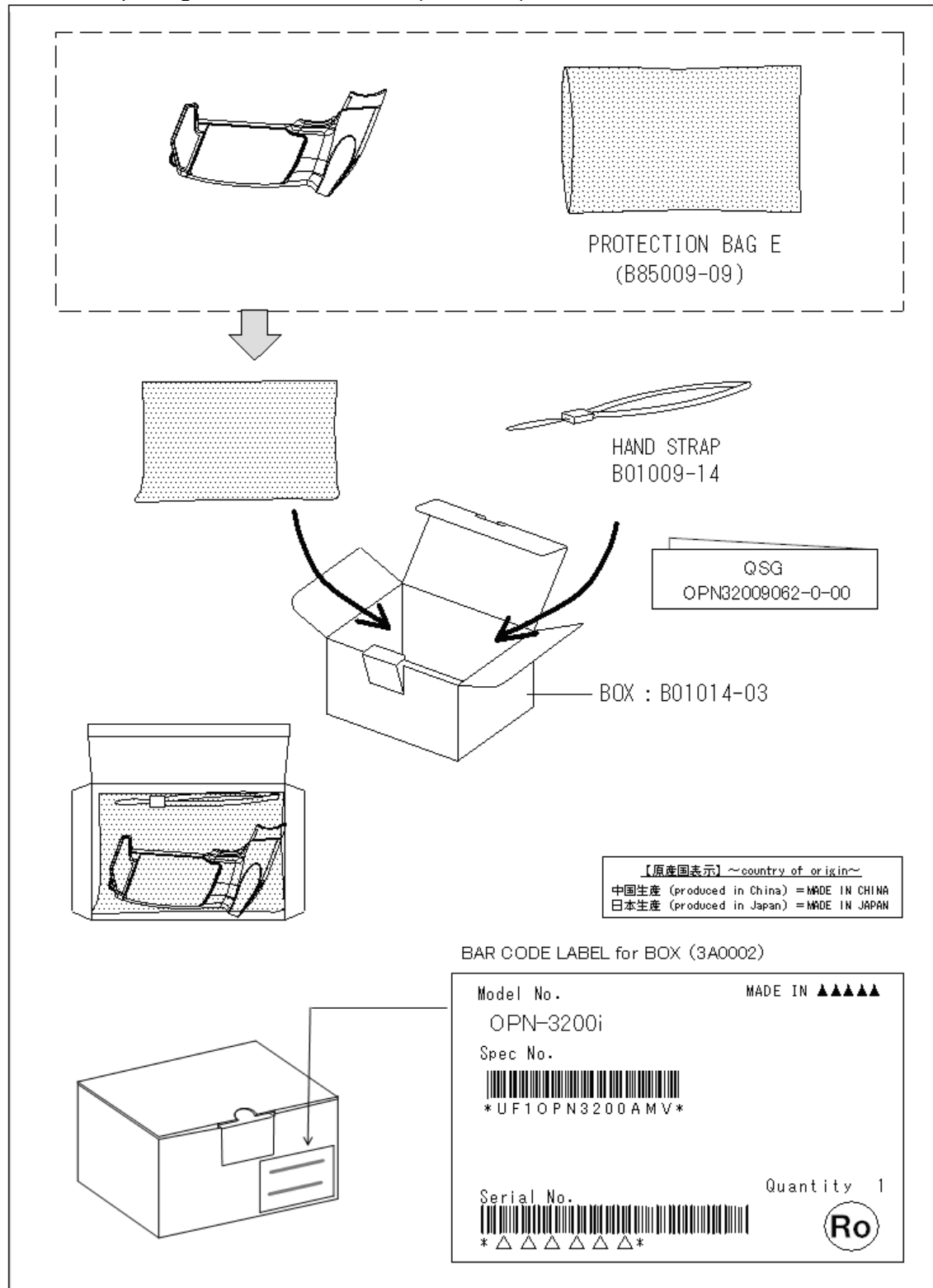
Figure 12: Individual Packaging
