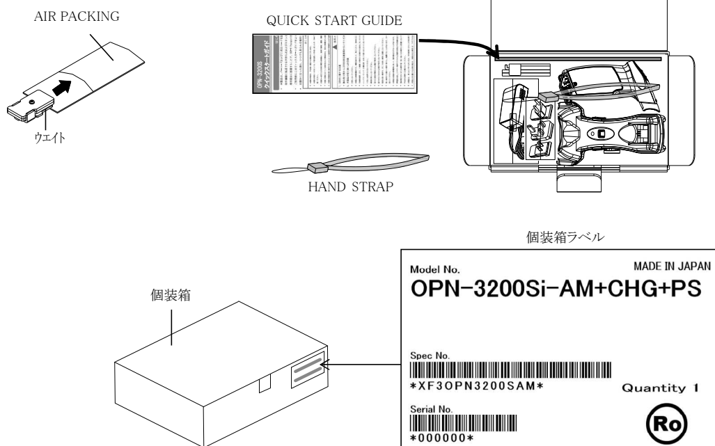
Figure 13: Individual Packaging
