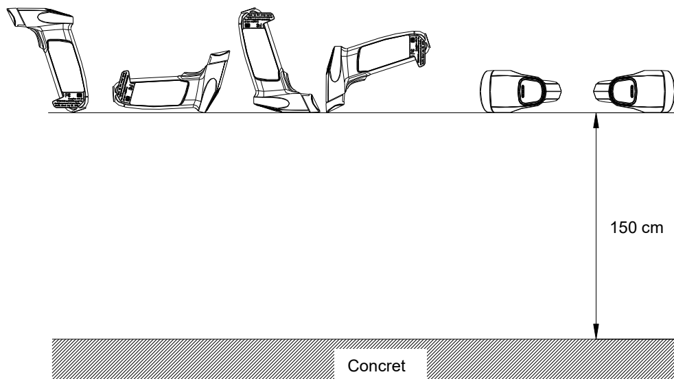
Figure 11: Drop Test
