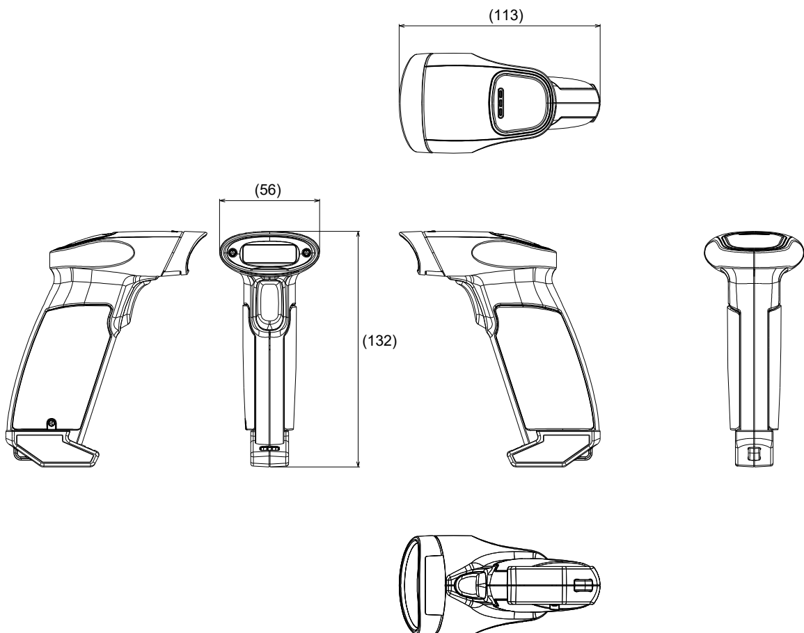
Figure 15: Mechanical Drawing
