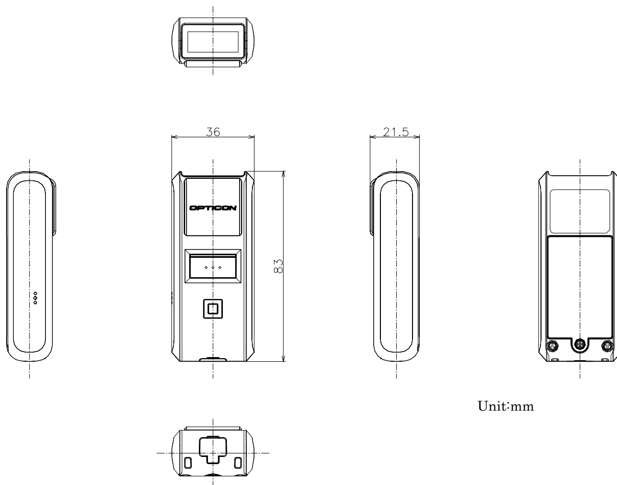
Figure 14: Outline drawing
