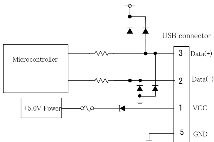
Figure 3:USBInterface Circuit
