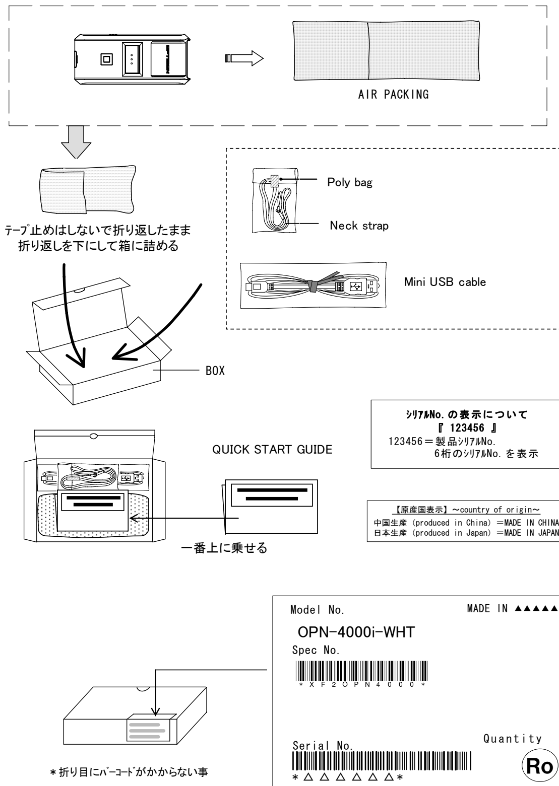
Figure 12: 個装梱包図
