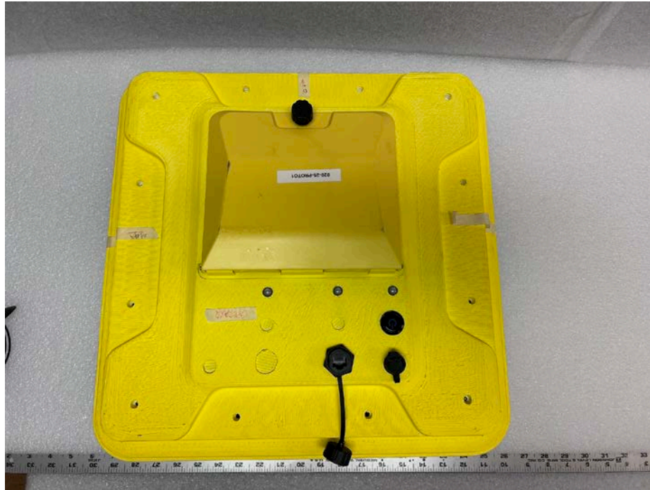
Non-Detachable Battery Cover Closed
