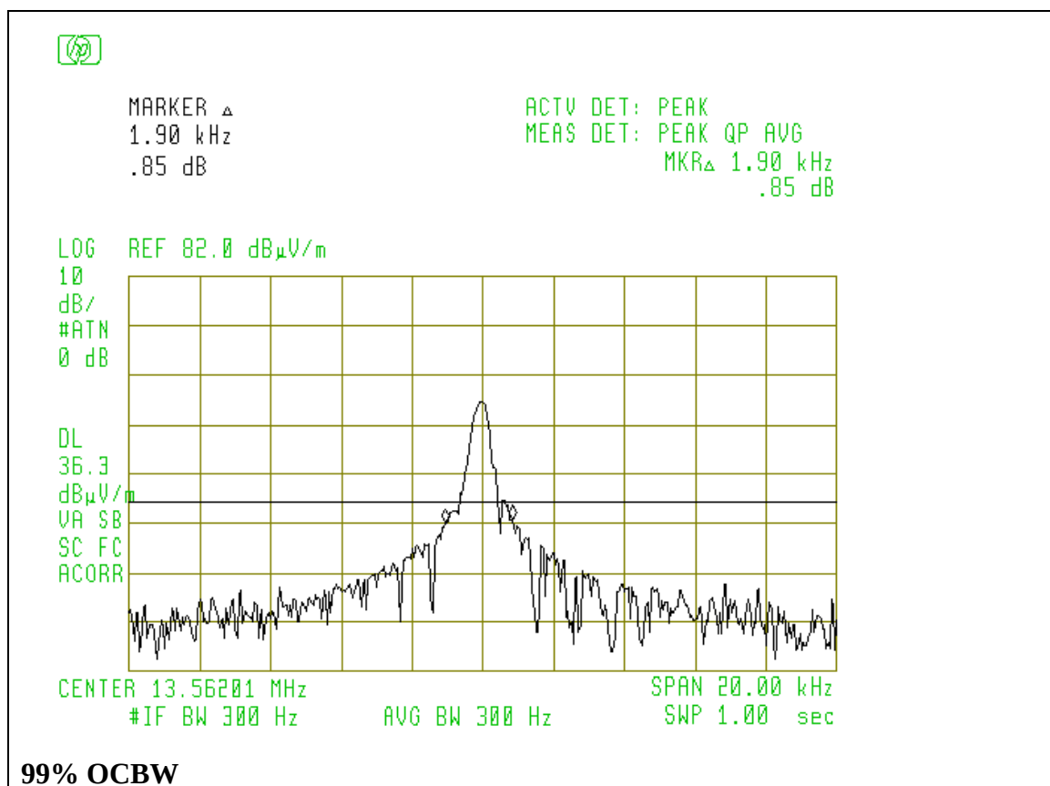
Figure 6.1 Occupied Bandwidth
