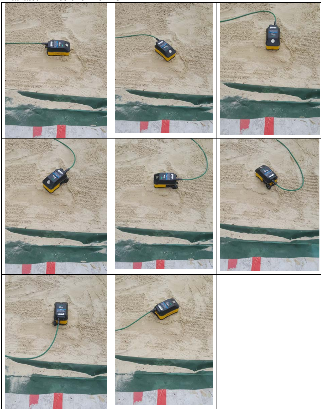
EUT Positions with 45 Degree Interval
