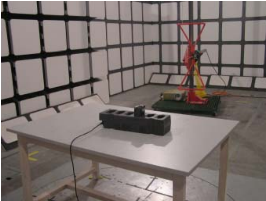
Charging Transmitting Mode: Radiated Emission - Front View (up to 1GHz)
