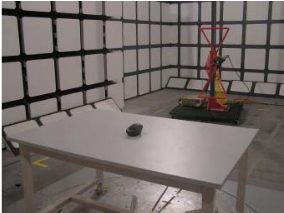
Transmitting Mode: Radiated Emission - Front View (up to 1GHz)
