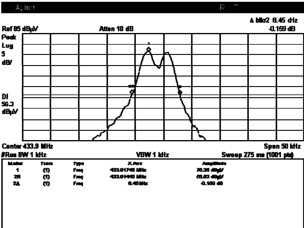
Plot of the Occupied bandwidth
