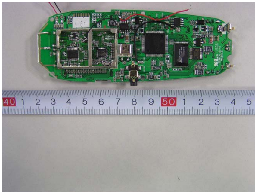
EUT – PCB Uncover of Shield Front View
