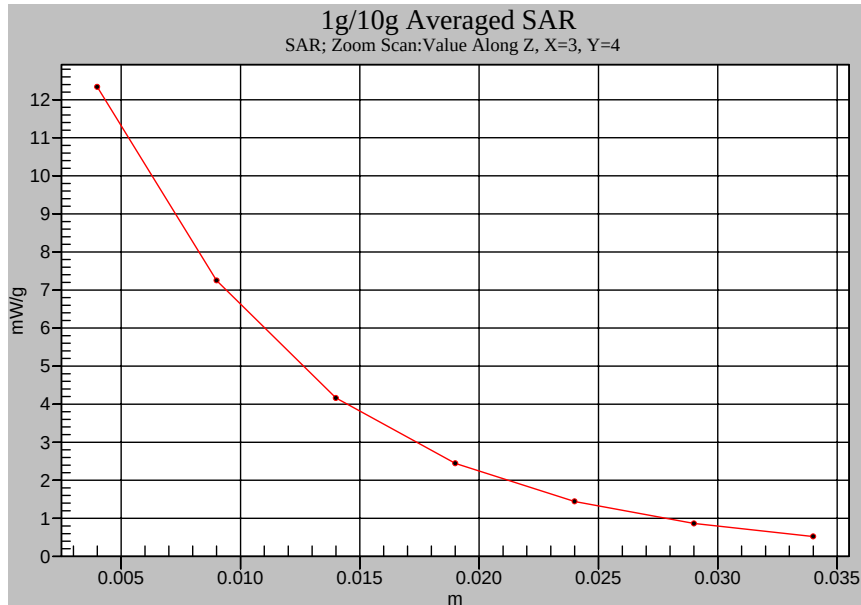
Head-Tissue-Simulating-Liquid 2GHz
