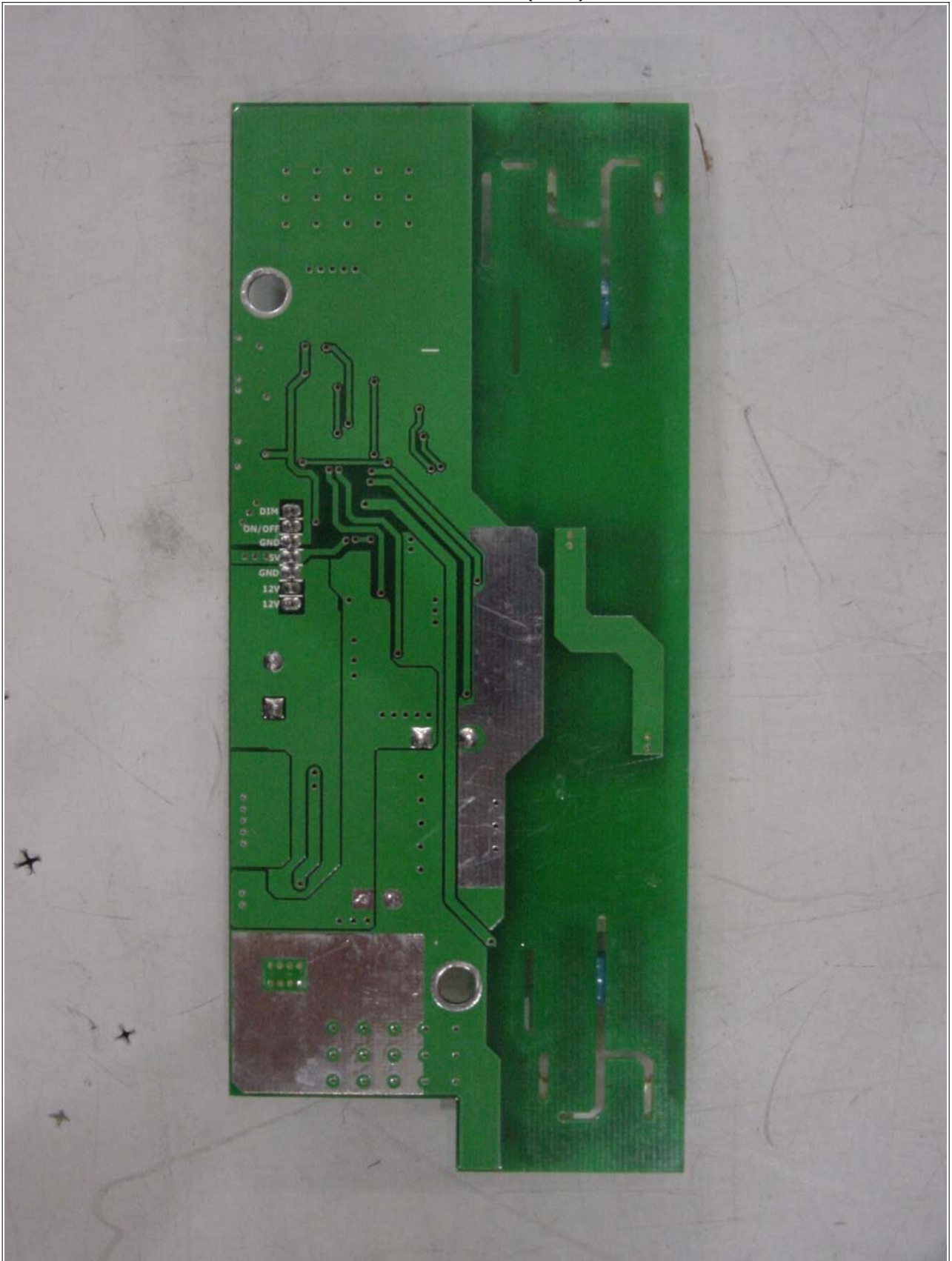
Inverter Board (Rear)
