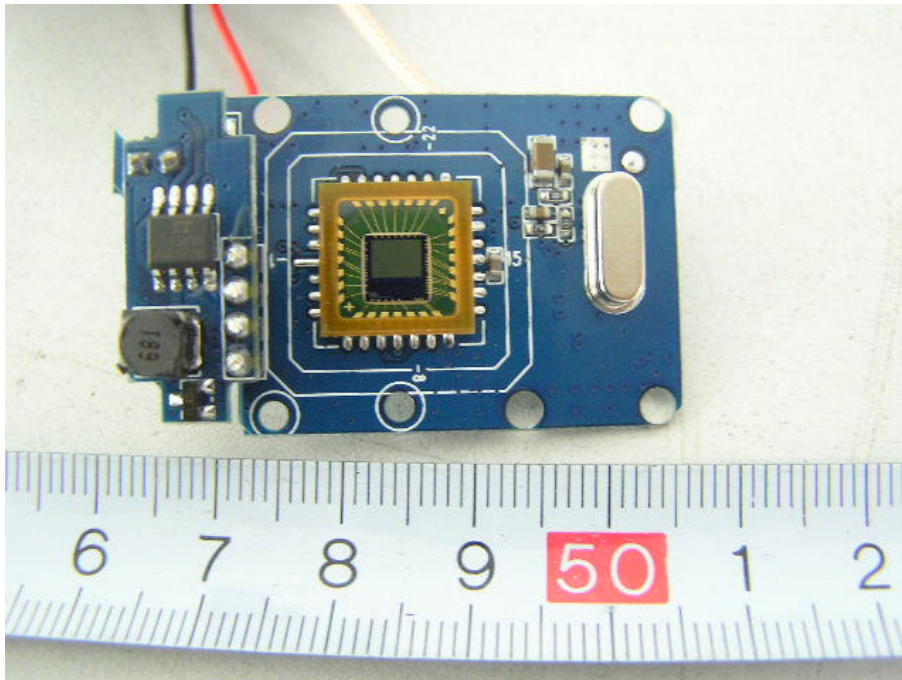
EUT-PCB View (2)
