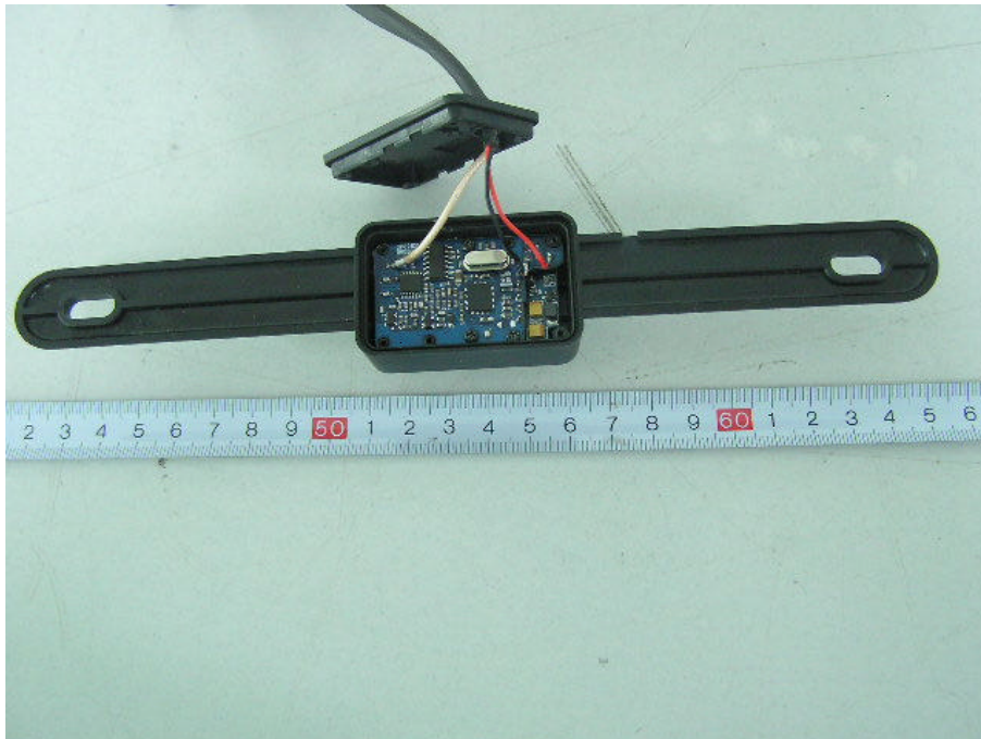
EUT-PCB View (1)
