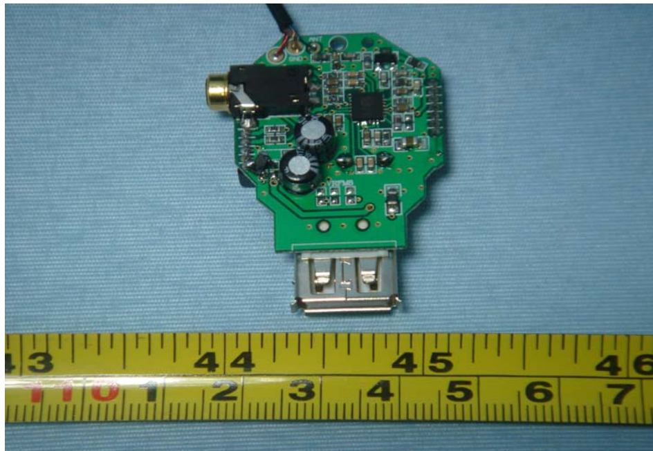
PCB2-Back View
