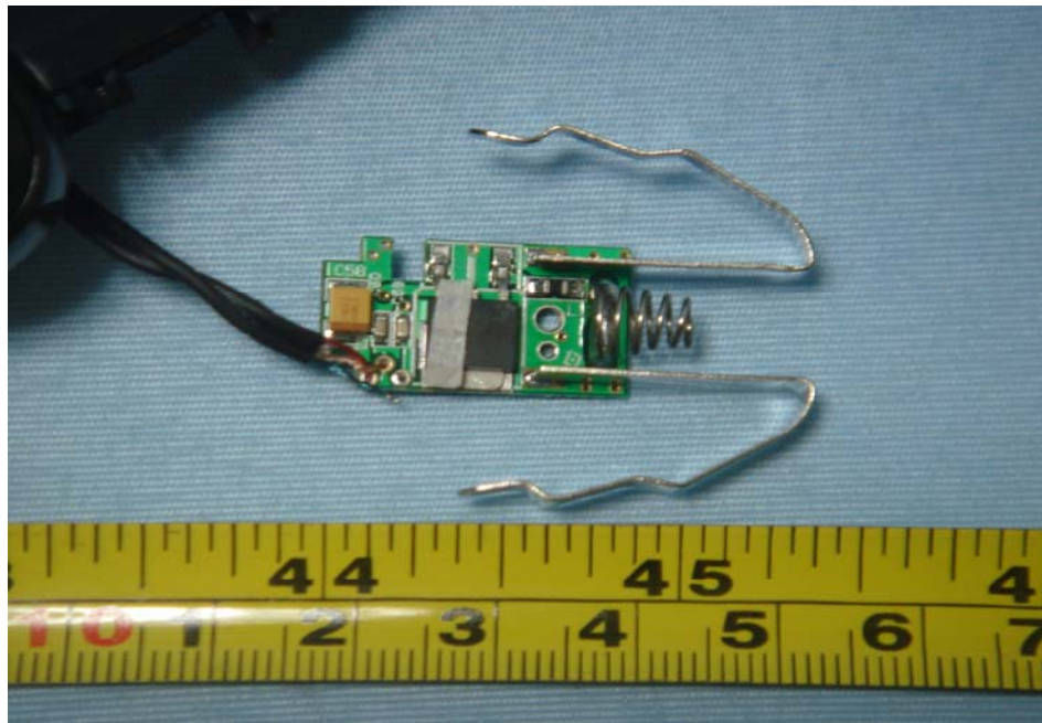
PCB3-Back View
