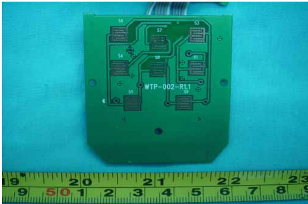
PCB1-Front View
