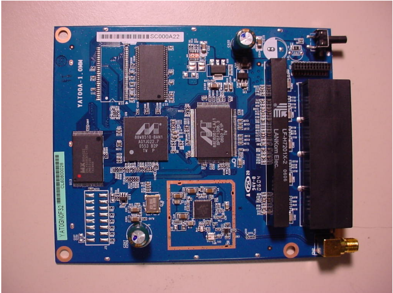
Figure 3: Internal Photographs – Top – Shield Removed
