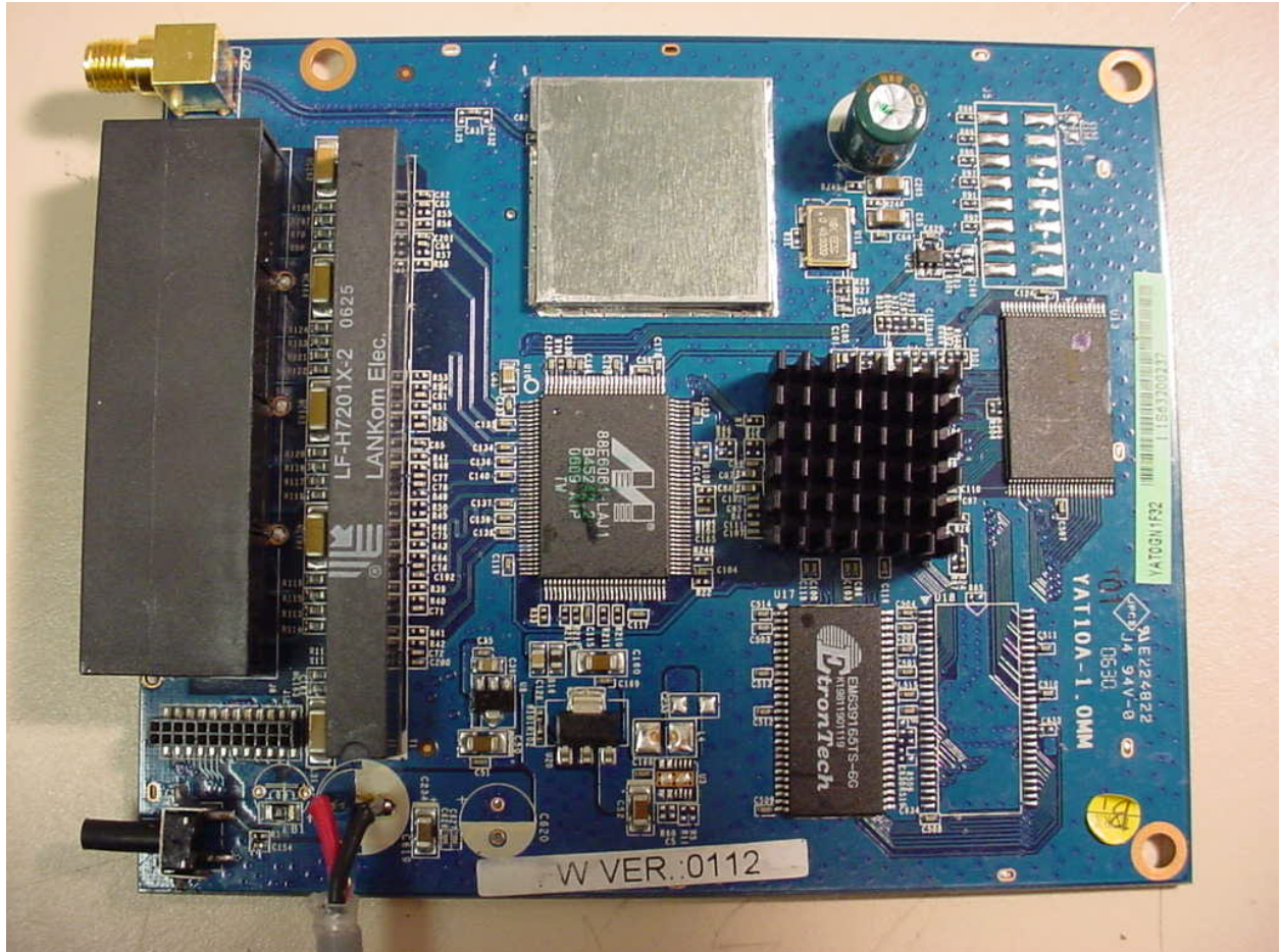
Figure 2: Internal Photographs - Top
