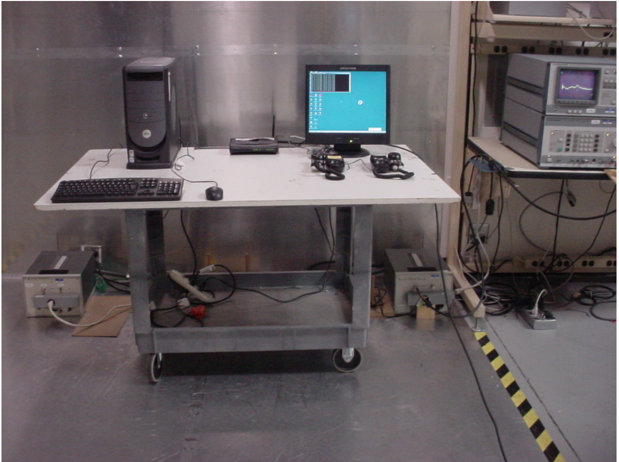
Figure 3: Conducted Emissions
