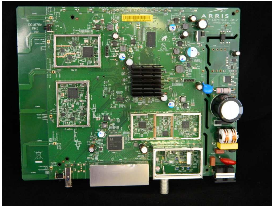
Figure 3: Internal Photo – DG1670A – Shields Removed
