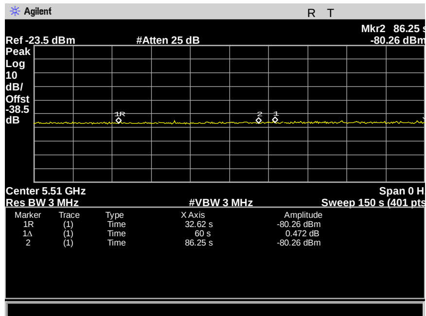
Figure 45: Radar Burst at the End of CACT
