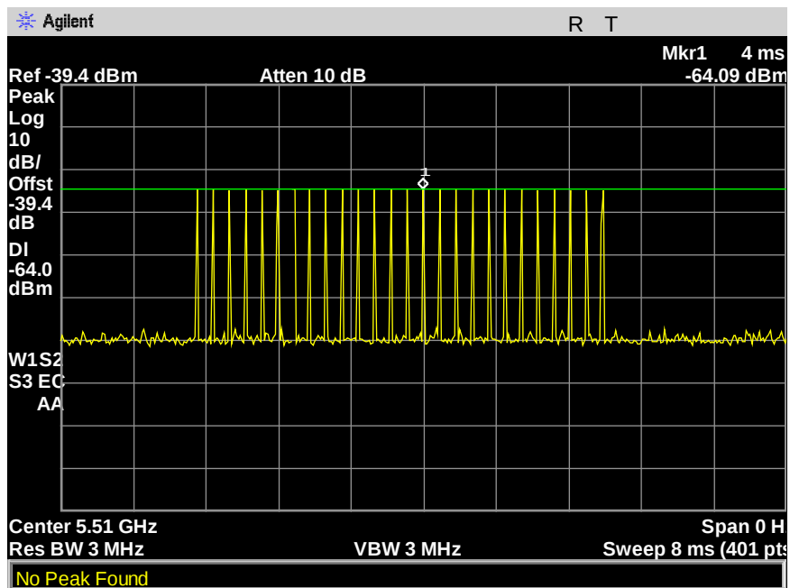
Figure 26: Radar Waveform Calibration, 5510 MHz calibration Type -2
