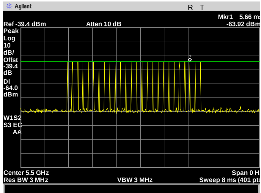
Figure 19: Radar Waveform Calibration, 5500 MHz calibration Type -2
