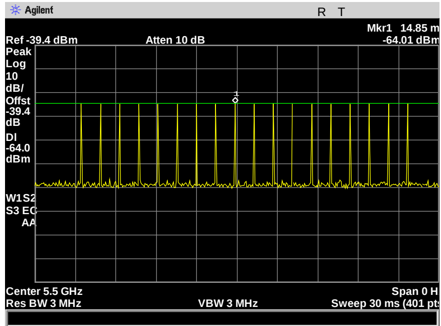
Figure 17: Radar Waveform Calibration, 5500 MHz calibration Type -0
