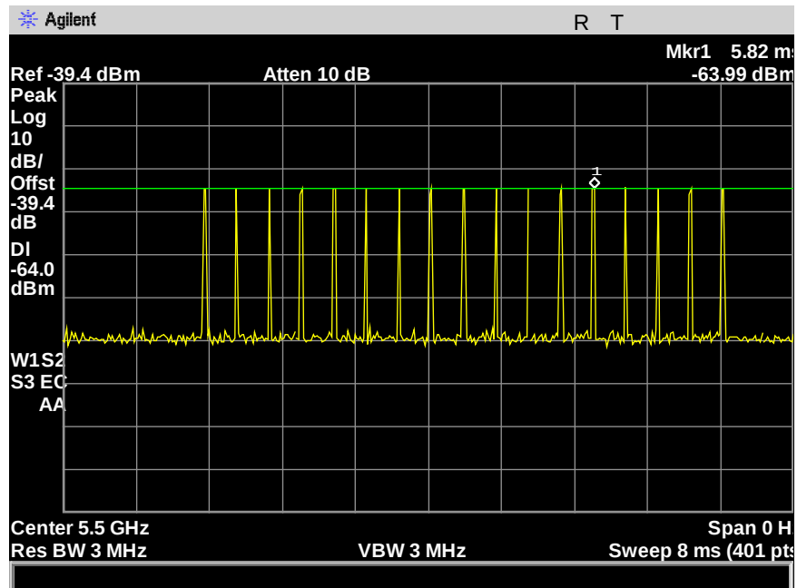
Figure 20: Radar Waveform Calibration, 5500 MHz calibration Type -3
