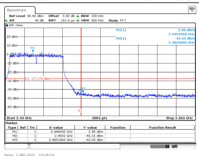
802.11ax (40 MHz) / Ant. 2 / 2452 MHz (Band Edge)
