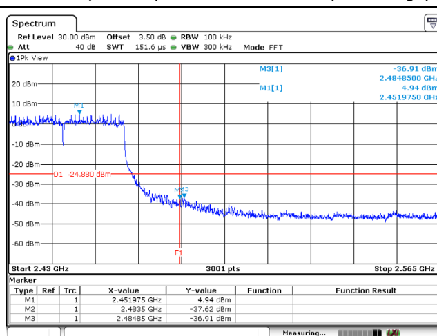
802.11ax (40 MHz) / Ant. 1 / 2447 MHz (Band Edge)
