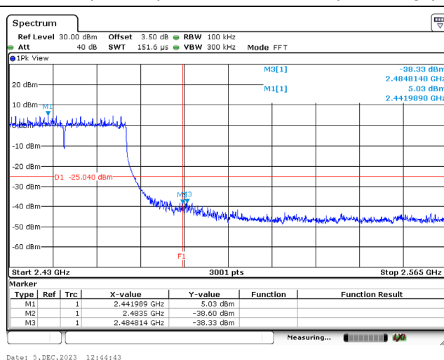
802.11ax (40 MHz) / Ant. 2 / 2447 MHz (Band Edge)
