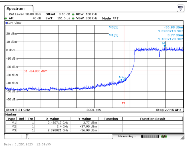
802.11ax (40 MHz) / Ant. 2 / 2427 MHz (Band Edge)
