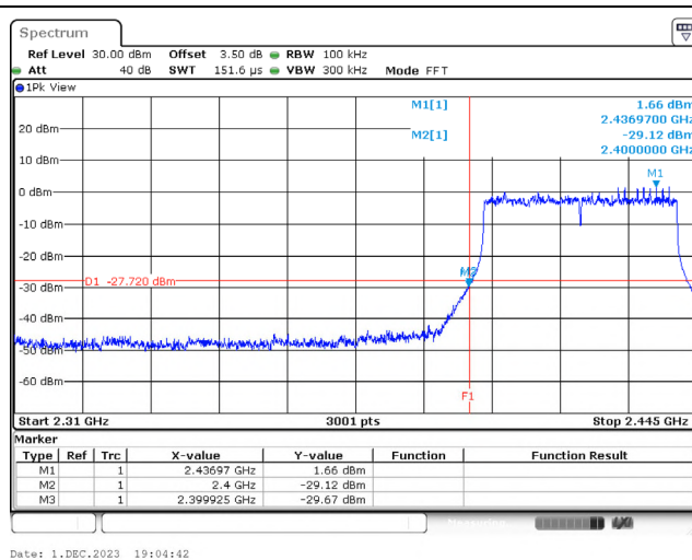
802.11ax (40 MHz) / Ant. 2 / 2422 MHz (Band Edge)
