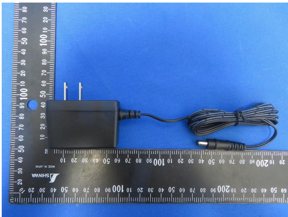
(10) EUT Photo (Adapter #2, M/N: WB-24M12FU)
