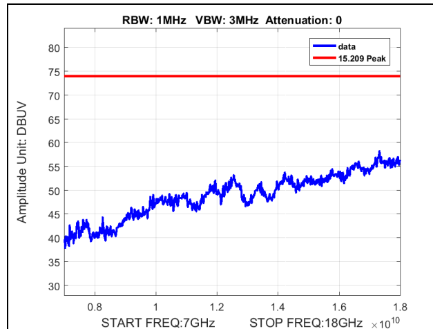
Plot 41. Radiated Spurious Emissions, Channel 5210 MHz, 802.11ac 80 MHz, 7 GHz – 18 GHz, Peak
