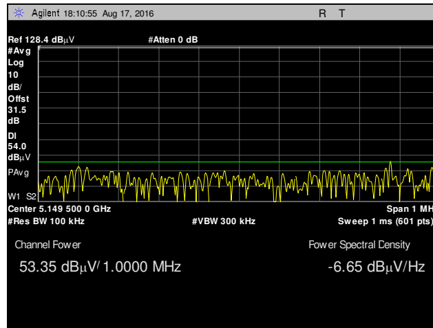
Plot 50. Radiated Band Edge, Integration Method, Channel 5180 MHz, 802.11n 20 MHz, t0 TP16.5, Average
