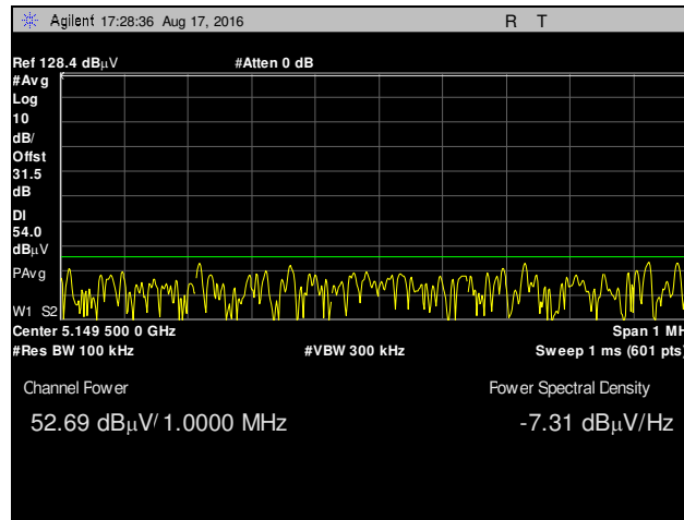
Plot 42. Radiated Band Edge, Integration Method, Channel 5180 MHz, 802.11a 20 MHz, r6 TP16.5, Average
