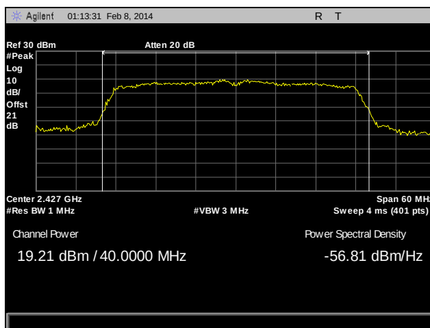
Plot 135. Peak Power Output, Channel 2, 802.11n 40 MHz, Ant. 1
