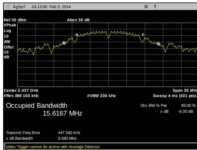
Plot 15. 6 dB Occupied Bandwidth, Channel 6, 802.11b, Ant. 1
