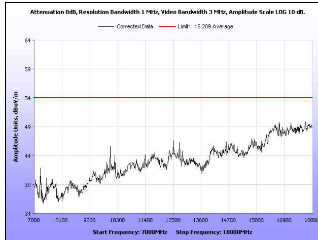
Plot 188. Radiated Spurious Emissions, Low Channel, 802.11g, Ant. 0, 7 GHz – 18 GHz
