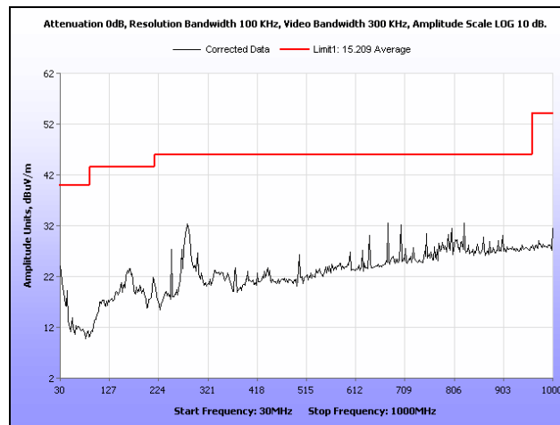
Plot 189. Radiated Spurious Emissions, Mid Channel, 802.11g, Ant. 0, 30 MHz – 1 GHz
