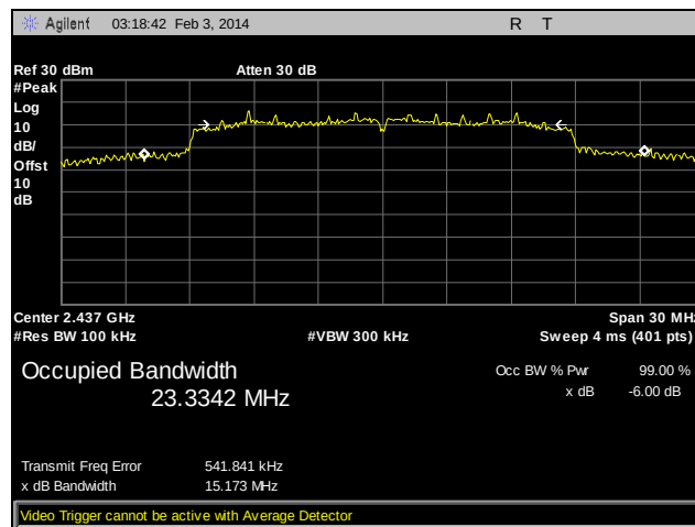
Plot 27. 6 dB Occupied Bandwidth, Channel 6, 802.11n 20 MHz, Ant. 1
