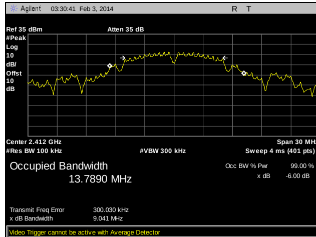
Plot 14. 6 dB Occupied Bandwidth, Channel 1, 802.11b, Ant. 1
