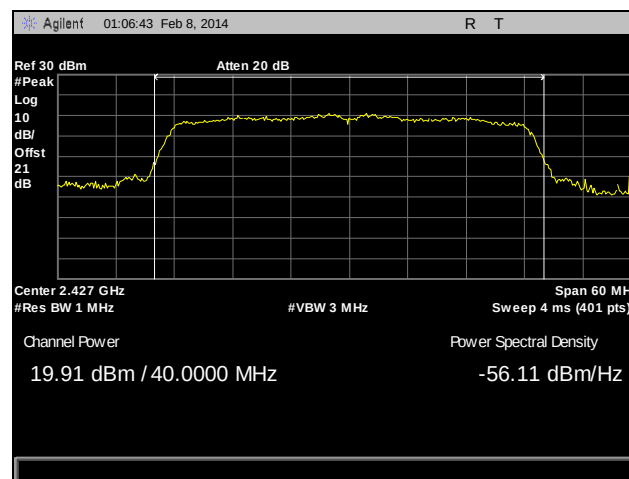
Plot 153. Peak Power Output, Channel 2, 802.11n 40 MHz, Ant. 1, MIMO
