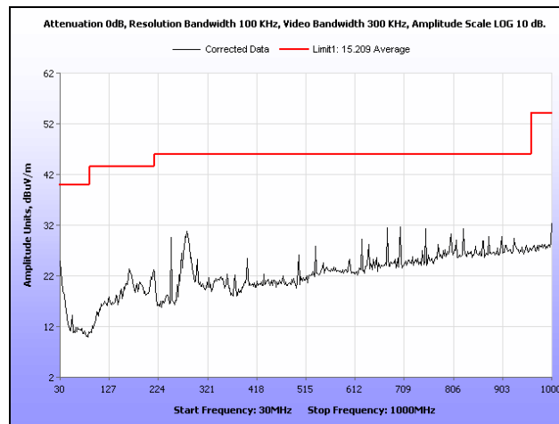
Plot 201. Radiated Spurious Emissions, Mid Channel, 802.11g, Ant. 1, 30 MHz – 1 GHz
