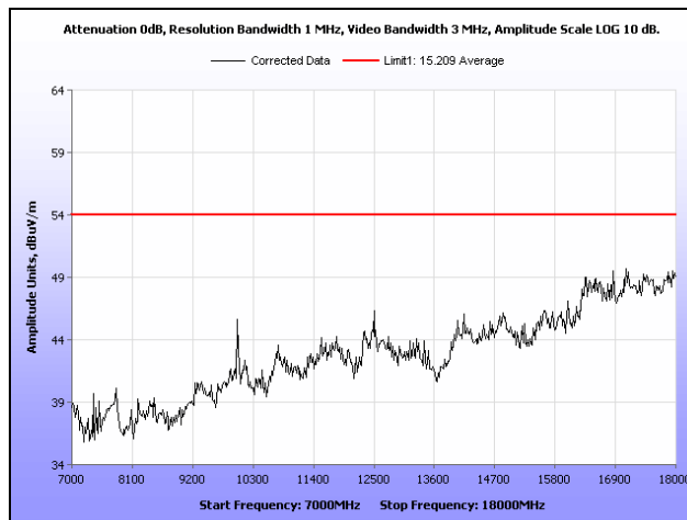
Plot 208. Radiated Spurious Emissions, High Channel, 802.11g, Ant. 1, 7 GHz – 18 GHz
