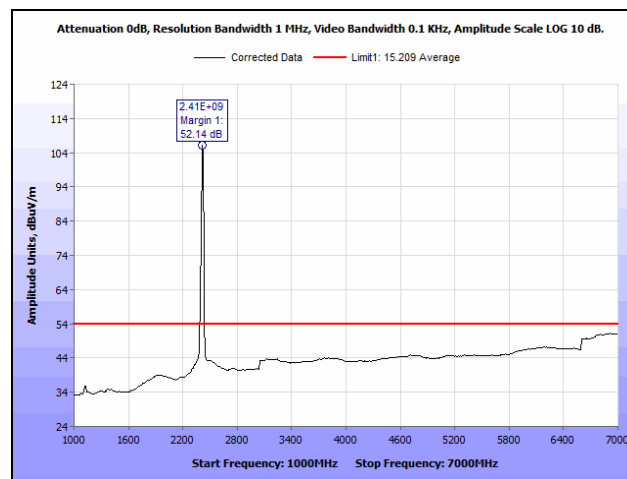
Plot 174. Radiated Spurious Emissions, Low Channel, 802.11b, Ant. 1, 1 GHz – 7 GHz, Average
