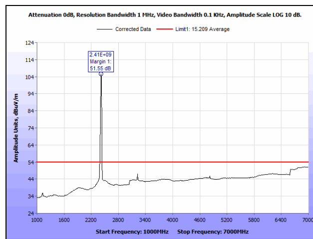
Plot 162. Radiated Spurious Emissions, Low Channel, 802.11b, Ant. 0, 1 GHz – 7 GHz, Average
