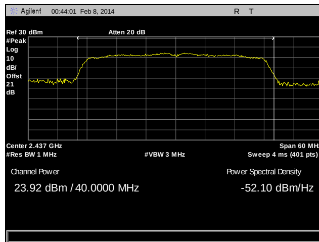
Plot 128. Peak Power Output, Channel 4, 802.11n 40 MHz, Ant. 0
