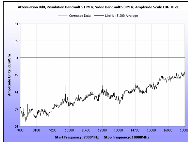
Plot 200. Radiated Spurious Emissions, Low Channel, 802.11g, Ant. 1, 7 GHz – 18 GHz
