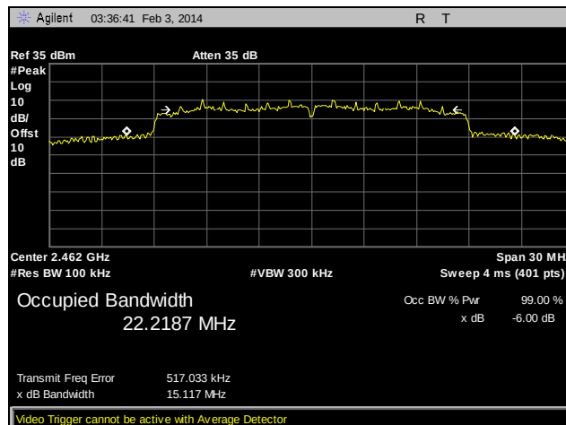
Plot 28. 6 dB Occupied Bandwidth, Channel 11, 802.11n 20 MHz, Ant. 1
