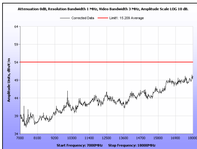
Plot 164. Radiated Spurious Emissions, Low Channel, 802.11b, Ant. 0, 7 GHz – 18 GHz
