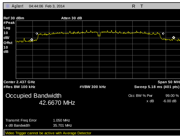
Plot 33. 6 dB Occupied Bandwidth, Channel 6, 802.11n 40 MHz, Ant. 1
