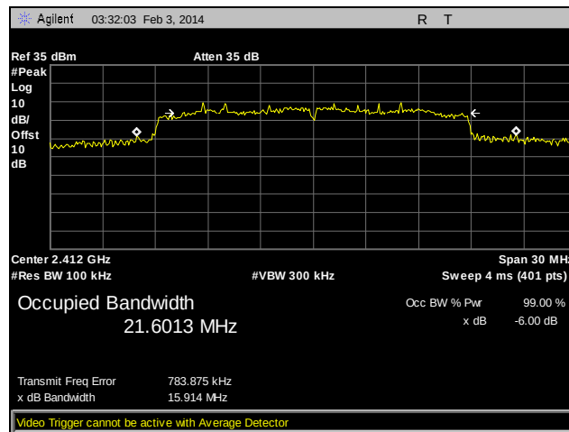
Plot 23. 6 dB Occupied Bandwidth, Channel 1, 802.11n 20 MHz, Ant. 0
