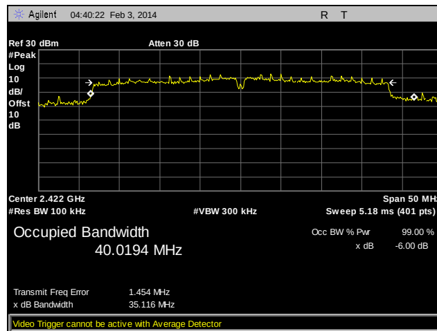
Plot 29. 6 dB Occupied Bandwidth, Channel 1, 802.11n 40 MHz, Ant. 0
