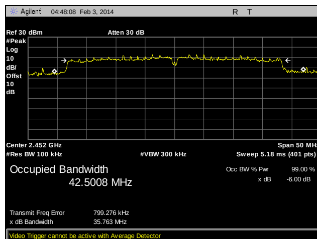
Plot 34. 6 dB Occupied Bandwidth, Channel 11, 802.11n 40 MHz, Ant. 1
