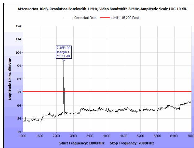
Plot 183. Radiated Spurious Emissions, High Channel, 802.11b, Ant. 1, 1 GHz – 7 GHz, Peak
