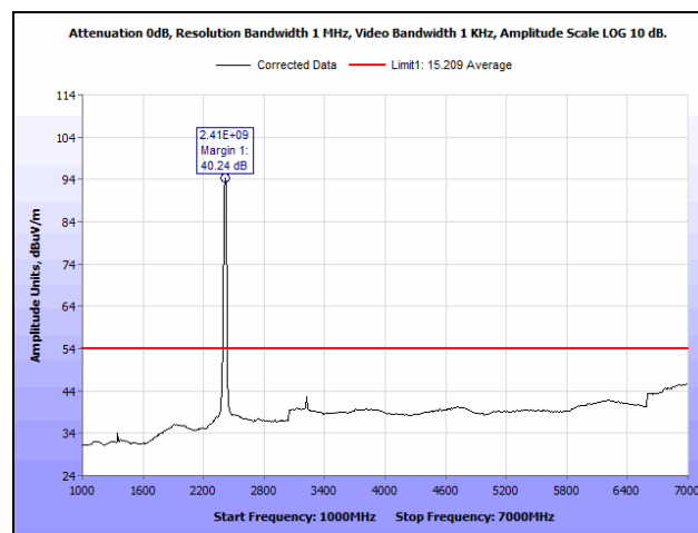
Plot 186. Radiated Spurious Emissions, Low Channel, 802.11g, Ant. 0, 1 GHz – 7 GHz, Average
