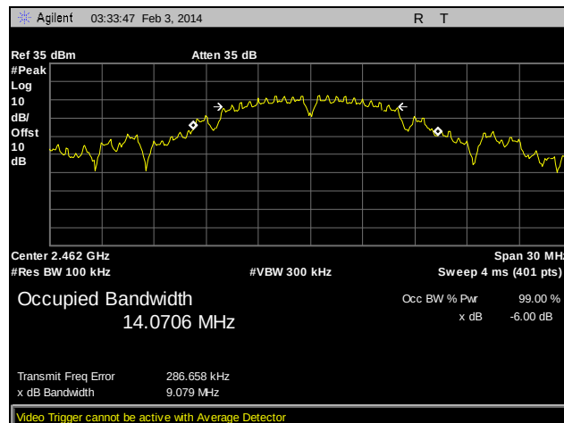
Plot 16. 6 dB Occupied Bandwidth, Channel 11, 802.11b, Ant. 1
