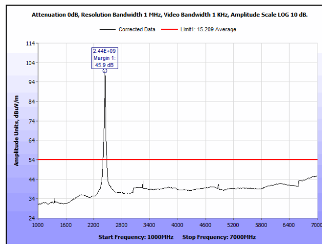
Plot 202. Radiated Spurious Emissions, Mid Channel, 802.11g, Ant. 1, 1 GHz – 7 GHz, Average
