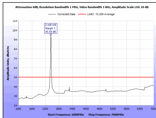
Plot 190. Radiated Spurious Emissions, Mid Channel, 802.11g, Ant. 0, 1 GHz – 7 GHz, Average
